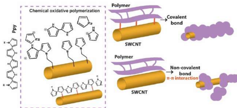
Figure 10. Schematic representation of the reaction mechanism and covalently and non-covalently final nanocomposites.
