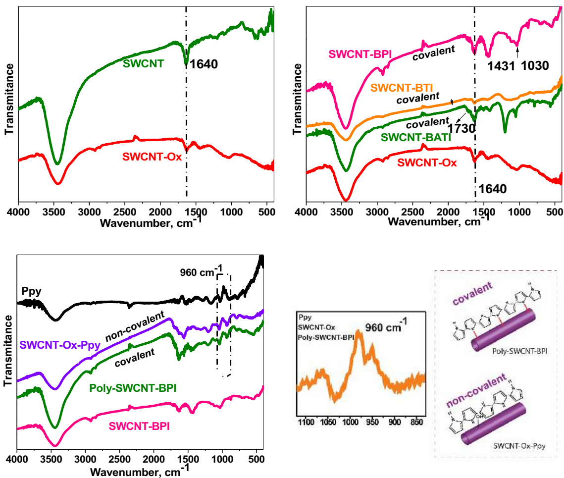
Figure 7. FTIR transmission spectra of functionalized samples (SWCNT-Ox, SWCNT-BATI, SWCNT-BPI) and the covalently and non-covalently linked nanocomposites (Poly-SWCNT-BPI and SWCNT-Ox-Ppy).
