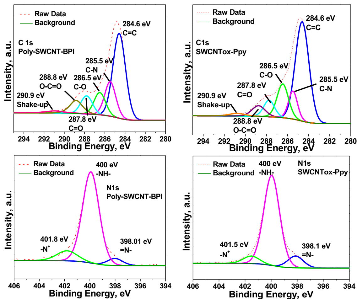
Figure 5. High-resolution C1s and N1s XPS spectra of Poly-SWCNT-BPI and SWCNT-Ox-Ppy.
