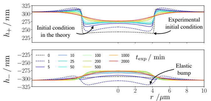
Figure 2. AFM profiles of the top and bottom interfaces of a free-standing hole with h_2 = 80 nm, h_0 = 610 nm, and r_0 = 4.2 \mu\text{m} (see Fig. 1), at various annealing times t_{\text{exp}} as indicated. An “elastic bump” is seen at t_{\text{exp}} = 1 min due to the residual stresses in the film from the sample preparation. The viscous model takes the profiles at 5 min as initial profiles, in order to ignore any prior elastic effect.
