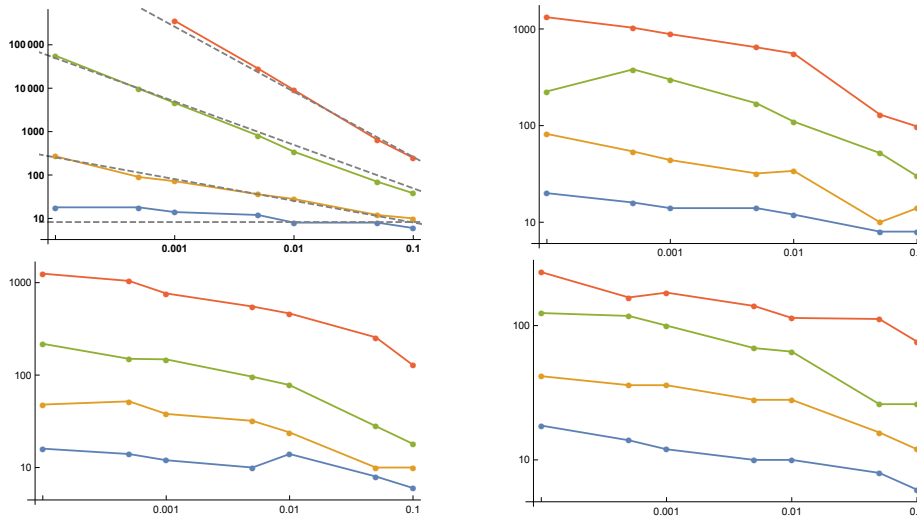
Figure 4: Solving time in seconds (in ordinate) depending on the precision (in abscissa) and the dimension ( n=2 in blue, n=3 in yellow, n=4 in green, n=5 in red). Upper-left: branch-and-bound without any anti-clustering technique. Upper-right: branch-and-bound with the lower-bounding technique described in Section 3.2. Lower-left: branch-and-bound with the first-order rejection technique described in Section 3.1. Lower-right: branch-and-bound with both techniques.
