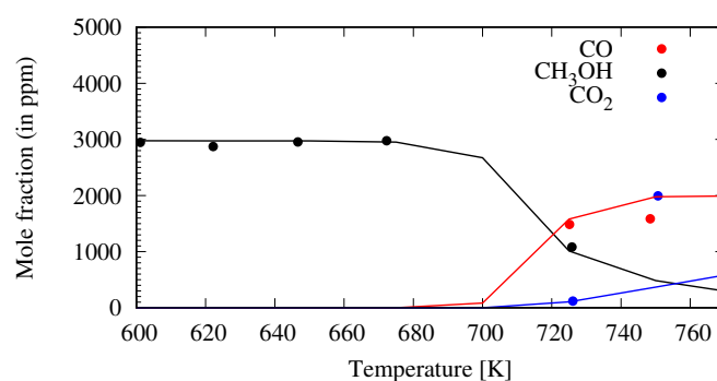
Fig. C.4. Reaction profiles of \text{CH}_3\text{OH} /air mixtures in a flow reactor, where symbols represent the experimental data of Held & Dryer (1994) and curves modeling results using the chemical scheme of Venot et al. (2012) (dashed lines) and with the updated chemical scheme of this paper (solid lines). Experimental conditions: 0.33 mol% \text{CH}_3\text{OH} + 0.6 mol% \text{O}_2 + \text{N}_2 , T around 1000 K, P = 0.25 MPa.
