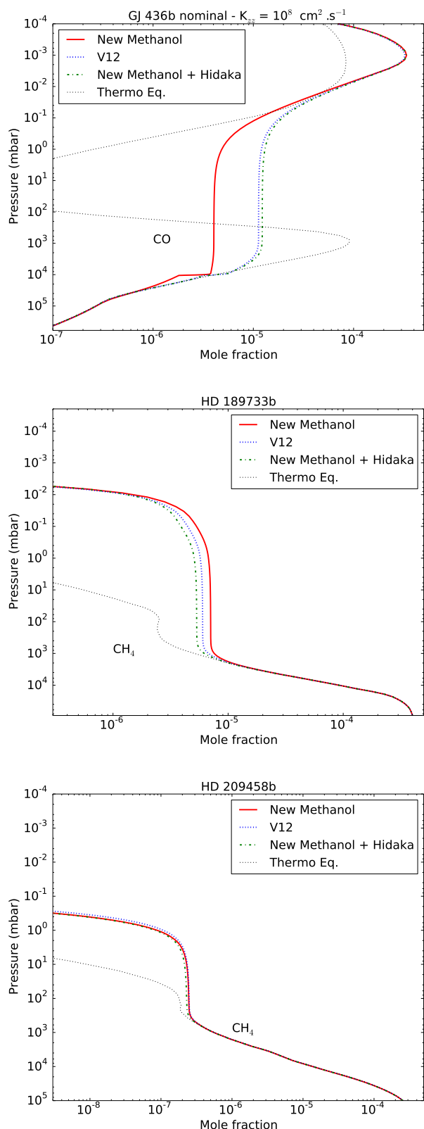
Fig. 8. Vertical abundances profiles of CO in GJ 436b (top) and of CH 4 in HD 189733b (middle) and in HD 209458b (bottom) using different chemical schemes, as labeled.
