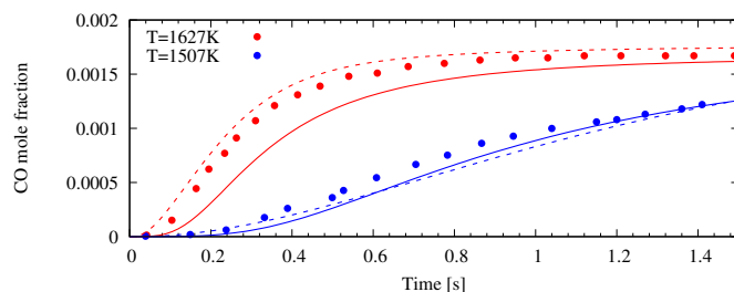
Fig. C.3. Mole fraction of methanol ( top ) and carbon monoxide ( bottom ) versus time for the combustion of methanol in a shock tube for a pressure around 2.5 atm, and an equivalence ratio of 1. The points represent experimental data from Ren et al. (2013) , and the lines show modeling results using the chemical scheme of Venot et al. (2012) (dashed) and with the updated chemical scheme of this paper (solid). P = 2.2 atm, (right) P = 1.1 atm.
