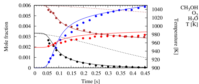
Fig. C.4. Reaction profiles of \text{CH}_3\text{OH} /air mixtures in a flow reactor, where symbols represent the experimental data of Held & Dryer (1994) and curves modeling results using the chemical scheme of Venot et al. (2012) (dashed lines) and with the updated chemical scheme of this paper (solid lines). Experimental conditions: 0.33 mol% \text{CH}_3\text{OH} + 0.6 mol% \text{O}_2 + \text{N}_2 , T around 1000 K, P = 0.25 MPa.
