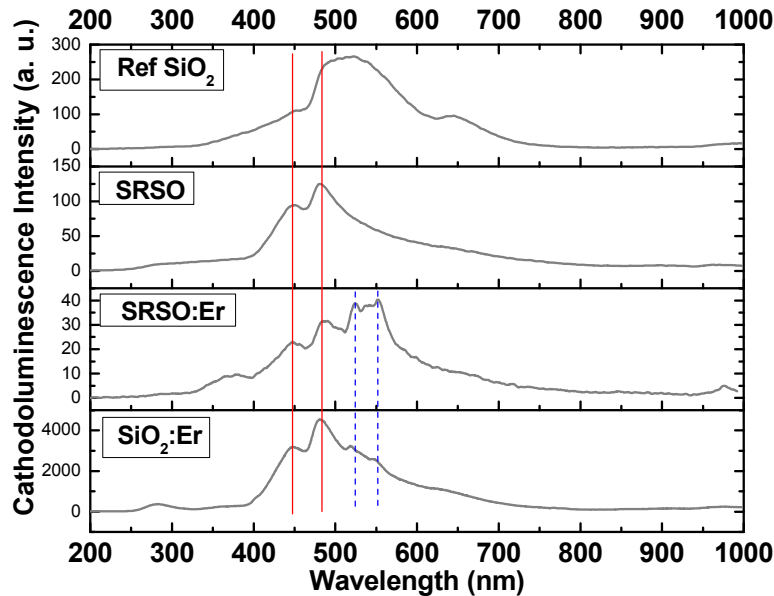
Figure 5. Cathodoluminescence spectra of (from the top to the bottom): a reference SiO 2 , SRSO sample, SRSO:Er sample and SiO 2 :Er. All these samples are non-annealed and were deposited at 500°C.
