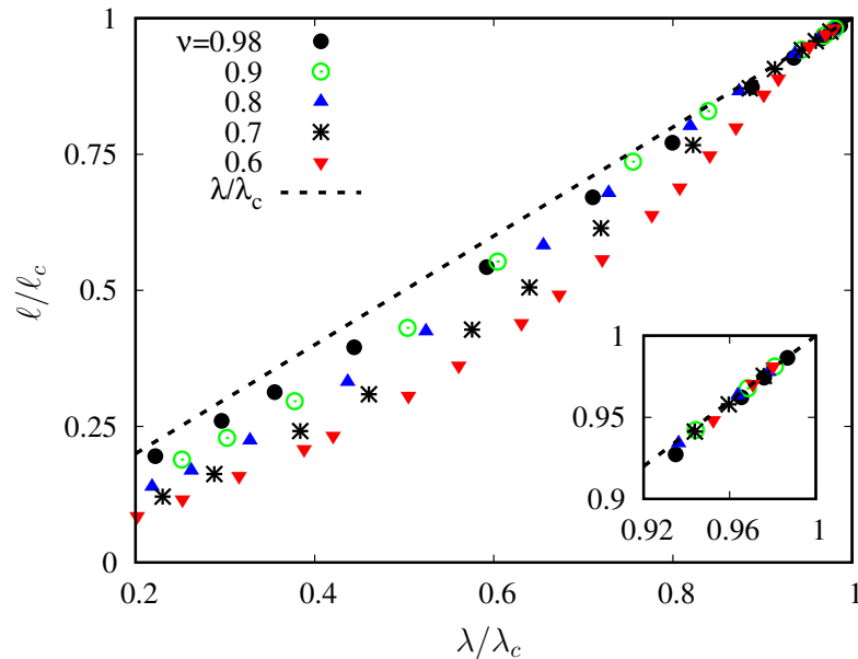
FIG. 8. Normalized vesicle length \ell/\ell_c versus the reduced radius ratio \lambda/\lambda_c for a wide range of reduced volumes \nu ( C_{\text{aB}} = 50 ), together with the linear scaling \ell/\ell_c = \lambda/\lambda_c (Eq. (26)).
