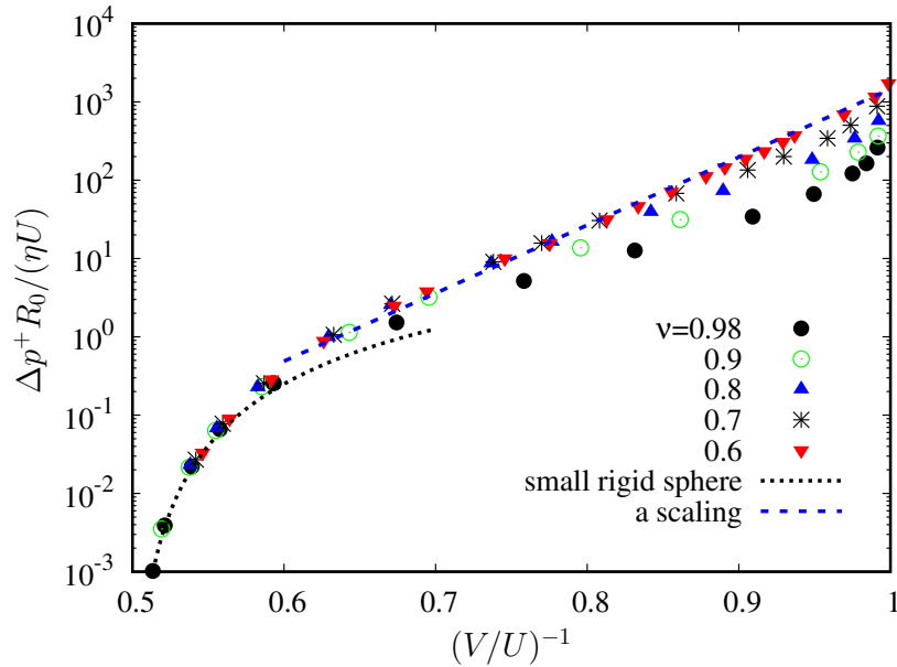
FIG. 12. Dimensionless pressure drop \Delta p^+ R_0 / (\eta U) versus the reciprocal of the relative velocity V/U . The dotted curve shows the analytical prediction for a small rigid sphere (29). The dashed line is the best fitting (30) to \nu = 0.6 in the range of 0.6 < (V/U)^{-1} < 0.995 .
