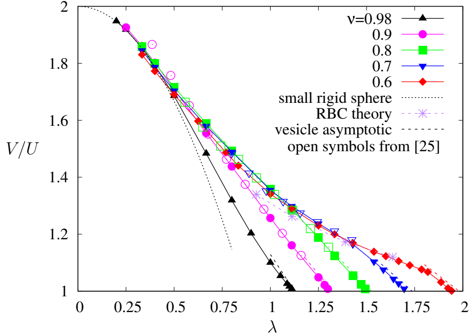
FIG. 9. Variation of the relative velocity V/U as a function of the confinement \lambda for a wide range of reduced volumes \nu ( Ca_B = 50 ). The filled symbols represent the present numerical results with the open symbols of the same shape and color for the 3D numerical results of [25] (figure 10, \nu = 0.9, 0.8 , and 0.7 ). Also shown are the asymptotic prediction for a small rigid sphere moving along the centreline of a tube (27a) (dotted line), the asymptotic predictions of (28a) (dashed lines colored differently according to the appropriate reduced volume), and the prediction of a lubrication model for red blood cells [34] (RBC theory).
