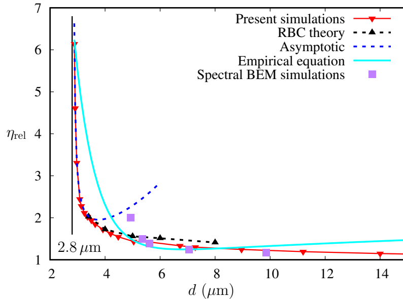
FIG. 13. Variation of relative apparent blood viscosity \eta_{\text{rel}} with tube diameter d in \mu\text{m} for a hematocrit H_T of 0.45. Curve -\blacktriangledown- represents simulation results based on single-file fluid model, and curve -\blacktriangle- represents lubrication model of RBCs [34]. Dashed line in blue shows asymptotic theory for dimensionless extra pressure drop [32] (Eq. (28b)). Solid curve in cyan represents a fitting empirical equation to in-vitro experimental data [1]. Also shown is the spectral 3D BEM simulations of Ref. [28] (for H_T = 0.30 ). The vertical line (black) indicates a lower limit ( d_c \simeq 2.8 \mu\text{m} ) to the diameter of tubes beyond which normal red blood cells cannot pass through without rupture.
