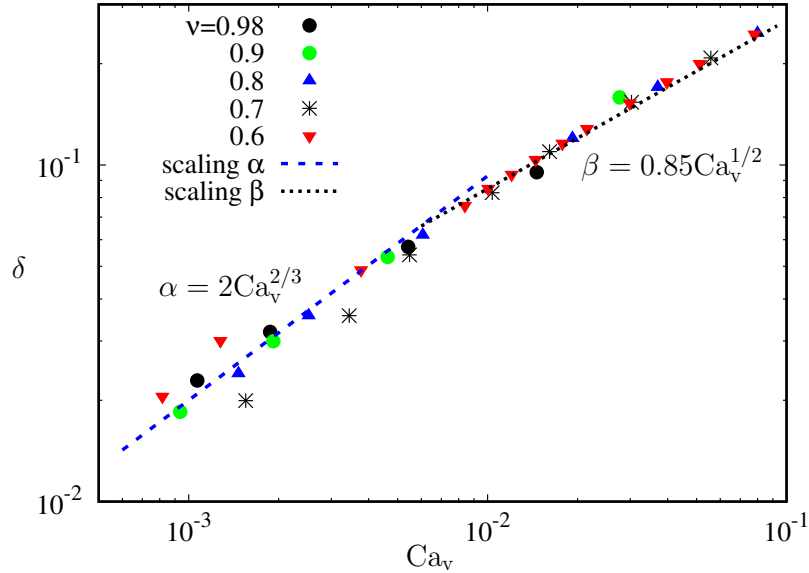
FIG. 7. The dimensionless thickness of the lubrication layer \delta plotted as a function of the capillary number Ca_v = \eta V / \gamma_F for a wide range of reduced volumes \nu , together with two scalings.
