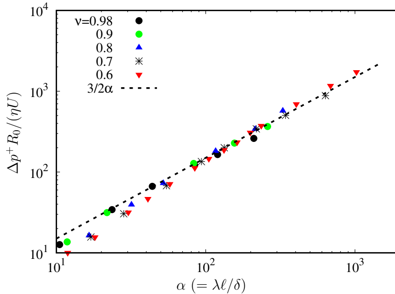
FIG. 11. Dimensionless pressure drop \Delta p^+ R_0 / (\eta U) plotted as a function of \alpha (= \lambda \ell / \delta) for highly confined vesicles (i.e., \lambda \rightarrow \lambda_c ). The dashed line shows the scaling 3/2\alpha .
