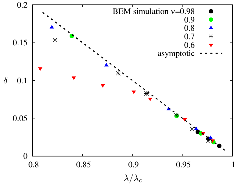
FIG. 6. The dimensionless thickness of the lubrication layer \delta plotted as a function of the reduced radius ratio \lambda/\lambda_c for a wide range of reduced volumes \nu ( Ca_B = 50 ), together with the asymptotic prediction (24).
