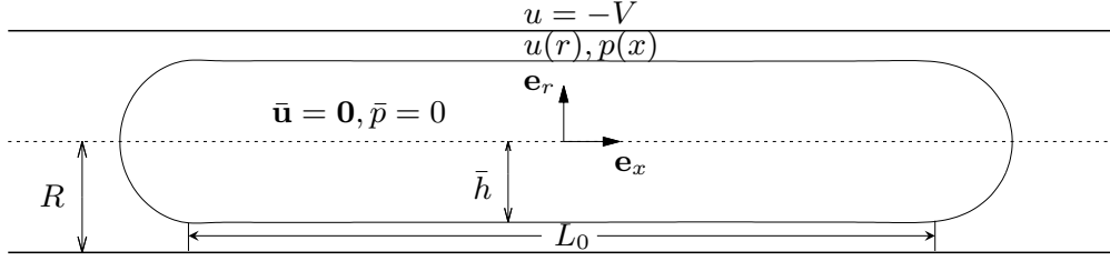
FIG. 14. Schematic of lubrication theory analysis for a steady, sphero-cylindrical vesicle moving along the axis of a circular tube of radius R . In a coordinate frame moving with the vesicle, there can be no flow and pressure gradient inside the vesicle. The vesicle has a cylindrical main body with a length L_0 , assumed large compared to R . Plotted vesicle profile corresponds to a vesicle shape for \nu = 0.6 , \lambda = 1.92 and Ca_B = 50 (shown in Fig. 3(d)); the tube wall is placed at more than 20% away from its actual place in order to amplify the width of the gap between the vesicle and the tube wall.
