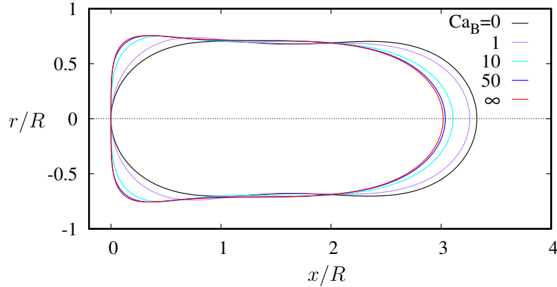
FIG. 2. Steady-state vesicle profile as a function of the bending capillary number Ca_B for \nu = 0.84 and \lambda = 1 .
