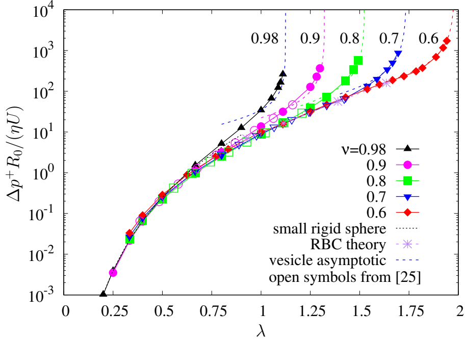
FIG. 10. Variation of the dimensionless pressure drop \Delta p^+ R_0 / (\eta U) as a function of the confinement \lambda for a wide range of reduced volumes \nu ( Ca_B = 50 ). The filled symbols represent the present numerical results with the open symbols of the same shape and color for the 3D numerical results of [25] (figure 11, \nu = 0.9, 0.8 , and 0.7 ). Also shown are the asymptotic prediction for a small rigid sphere moving along the centreline of a tube (27b) (dotted line), the asymptotic predictions of (28b) (dashed lines), and the prediction of a lubrication model for red blood cells [34] (RBC theory).
