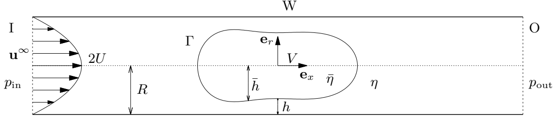
FIG. 1. Schematic illustration of a vesicle flowing along the centerline of a circular tube of radius R in a pressure-driven flow. The system is rotationally symmetric about the x -axis. The boundaries of the control volume ( D ) are the inlet and outlet sections I and O , the solid surface of the tube wall W , and the membrane/medium interface \Gamma , i.e., \partial D \equiv I \cup O \cup W \cup \Gamma . The vesicle shape and the gap size between the membrane and the tube wall are denoted by \bar{h} and h (\equiv R - \bar{h}) , respectively. The vesicle enclosed volume is denoted by \Omega .
