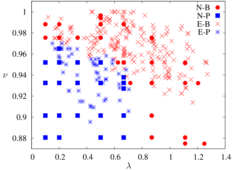
FIG. 4. Parachute-bullet phase diagram in the (\nu, \lambda) space. Filled symbols denote the present numerical results (● for bullet-like shape, ■ for parachute-like shape), crosses represent experimental data of Ref. [36] (× for bullet-like shape, * for parachute-like shape). Capillary number varies over four orders of magnitude ( 10^1 < Ca_B < 10^4 ).
