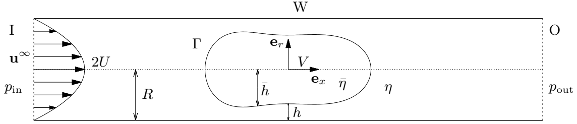
FIG. 1. Schematic illustration of a vesicle flowing along the centreline of a circular tube of radius R in a pressure-driven flow. The system is rotationally symmetric about the x -axis. The boundaries of the control volume ( D ) are the inlet and outlet sections I and O , the solid surface of the tube wall W , and the membrane/medium interface \Gamma , i.e., \partial D \equiv I \cup O \cup W \cup \Gamma . The vesicle shape and the gap size between the membrane and the tube wall are denoted by \bar{h} and h (\equiv R - \bar{h}) , respectively. The vesicle enclosed volume is denoted by \Omega .
