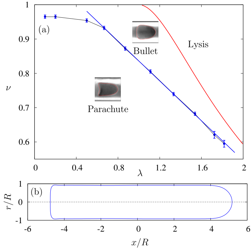
FIG. 5. (a) Shape transition line (blue) from parachute (low limit in error bars) to bullet (up limit in error bars) in the (\nu, \lambda) space ( C_{aB} = 50 ). Vesicles are flowing from left to right. The two typical vesicles are characterized, respectively, by \nu = 0.95 , \lambda = 0.8 and C_{aB} = 5 for the bullet-like shape, and \nu = 0.83 , \lambda = 0.67 and C_{aB} = 15 for the parachute-like shape. Insets show the comparison of the computed shapes (red line) with the reported ones in an experimental study [5]. The rupture line (red) represents the critical confinement \lambda_c (22). Membrane lysis occurs when \lambda > \lambda_c . (b) The shape at the parachute-bullet transition of a vesicle with the same typical deflation of red blood cells ( \nu = 0.6 ) flowing through a narrow capillary tube ( \lambda \simeq 1.8 ).
