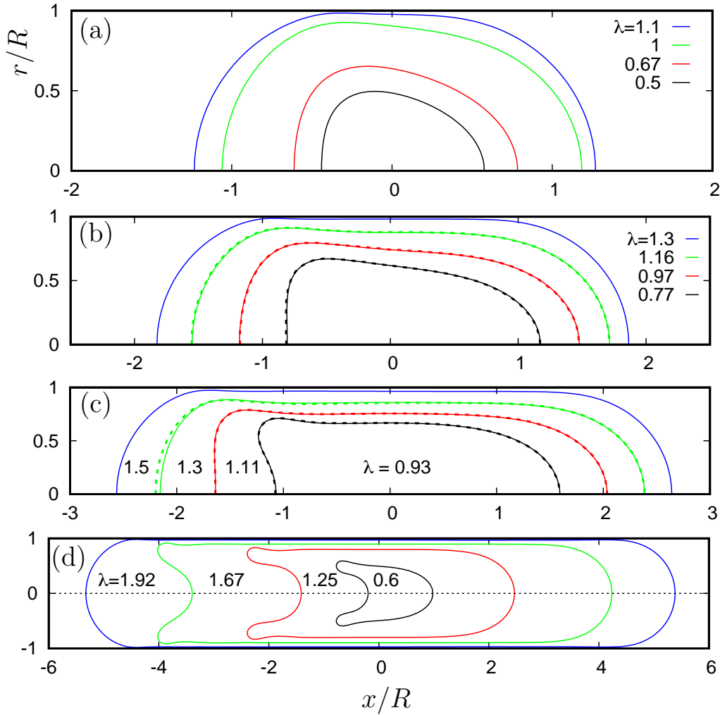
FIG. 3. Steady-state vesicle shapes (solid lines) as a function of the confinement \lambda for a wide range of reduced volumes \nu ( \text{Ca}_B = 50 ): (a) \nu = 0.98 , (b) \nu = 0.9 , (c) \nu = 0.8 , and (d) \nu = 0.6 . The dashed lines in (b) and (c) represent the 3D BEM simulations of [25], figure 9(b) ( \nu = 0.9 , \lambda_A = 1.2, 1, 0.8 ) and figure 9(c) ( \nu = 0.8 , \lambda_A = 1.4, 1.2, 1 ), respectively.
