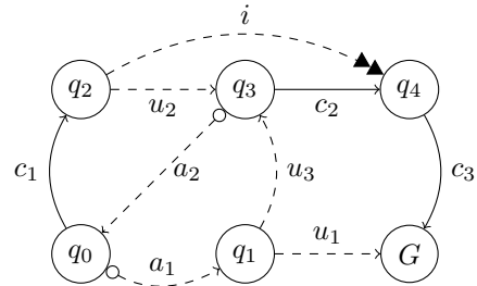
Figure 8. A reachability game. The objective is to reach the state G .
