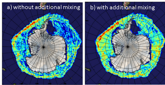
FIGURE 10 | Sensitivity of sea ice forecasting skill to ocean mixing around Antarctica. Weekly 7 days sea ice forecasts from the Global Ice-Ocean Prediction System (GIOPS) running operationally at the Canadian Centre for Meteorological and Environmental Prediction are evaluated against analyses over the year 2011. The evaluation of forecast skill is restricted to points where the analysis has changed by more than 10% over the forecast period (7 days). Warmer colors indicate larger root-mean squared error (maximum of 0.3 for dark red) with zero error shown as dark blue. Panels (a) and (b) show the forecast skill for experiments without and with additional ocean mixing respectively. Adapted from Smith et al. (2013).
