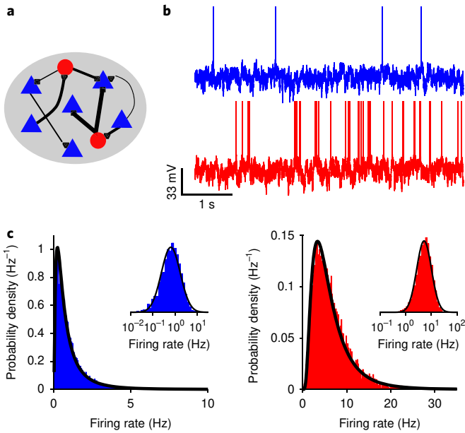
Fig. 1 | The spiking network model. a , A schematic drawing of the network of sparsely connected excitatory (blue triangles) and inhibitory (red circles) integrate-and-fire neurons. b , Membrane potential traces of randomly selected excitatory (blue) and inhibitory (red) neurons. c , The distributions of firing rates of the excitatory (blue) and inhibitory (red) neurons (estimated from a simulation of 3 min) in linear and logarithmic (inset) scales. Black lines are log-normal functions fitted to the (logarithmic) histograms (parameters of the fit: excitatory: mean, 1.01 Hz; variance, 1.03 Hz 2 ; inhibitory: mean, 6.41 Hz; variance, 16.27 Hz 2 ).
