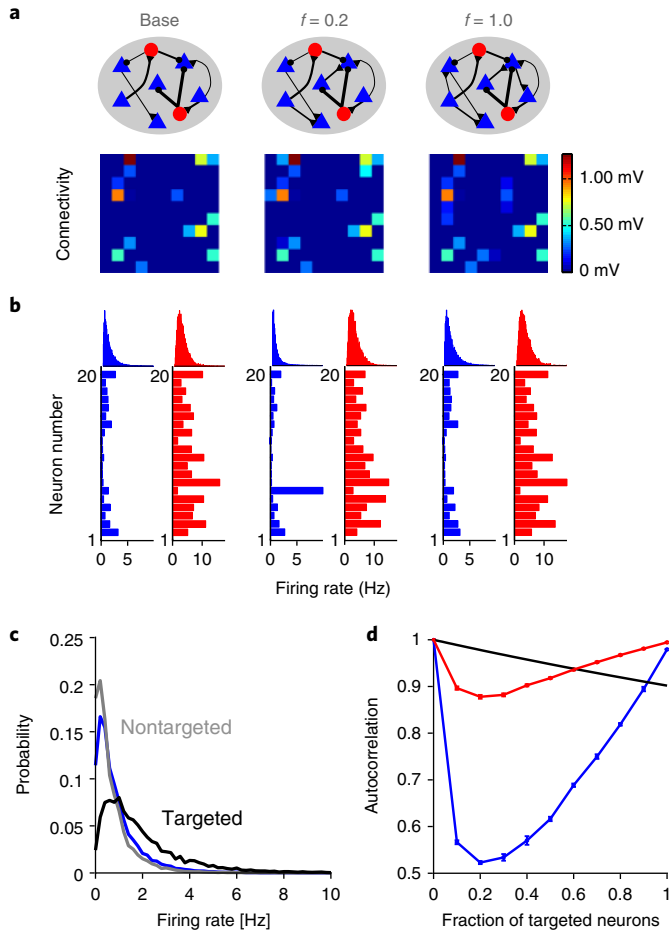
Fig. 7 | The effect of heterogeneous addition of E \rightarrow E connections. a , Top: schematic illustration of three sparsely connected networks of spiking neurons (see Methods). Left: baseline network, in which the probability of E \rightarrow E connection between each pair of neurons ( f ) is 0.2. Middle: the same network as in the left panel, in which randomly chosen 20% of the excitatory neurons are targeted: each targeted neuron is now connected to the 80% previously unconnected excitatory neurons with a probability of 5%, such that the overall probability of incoming E \rightarrow E connection to the targeted neurons is 24%. Connectivity onto nontargeted neurons is unchanged and their probability of incoming E \rightarrow E connection remains at 20%. Right: the same network when all excitatory neurons are targeted. Bottom: connectivity matrices between 10 randomly selected excitatory neurons given the conditions in the top row. b , Top: distributions of firing rates of excitatory (blue) and inhibitory (red) neurons given the conditions in a . Bottom: firing rates of randomly selected 20 excitatory (blue) and 20 inhibitory (red) neurons. c , Distributions of firing rates of the targeted (black) and nontargeted (gray) excitatory neurons when 20% of the neurons are targeted (middle panels in a and b . For comparison, the blue curve denotes the distribution of firing rates of the excitatory neurons in the random network (left panel in a ). d , Autocorrelogram of the E \rightarrow E connectivity matrices (black) and of the vectors of firing rates of excitatory (blue) and inhibitory (red) neurons as a function of the fraction of targeted neurons. Points denote average over five simulations; error bars are s.e.m.
