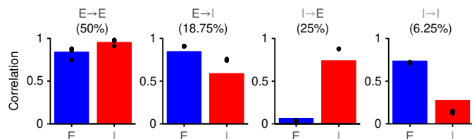
Fig. 3 | Rewiring different synaptic types differentially affects the patterns of network activity. Graphs present correlation coefficients of the firing-rate vectors before and after rewiring different synaptic types. Bars correspond to the theoretical prediction (see Methods); each of the five dots denotes the correlations computed from one numerical simulation (except E \rightarrow E , the five dots overlap). Numbers in brackets denote the fraction of corresponding synapses in the network.
