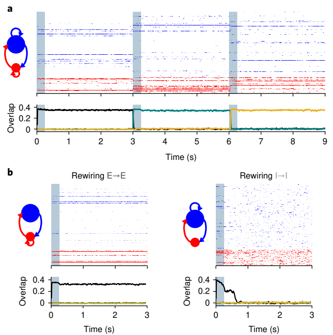
Fig. 5 | Synaptic rewiring and memory in a spiking network model. 2,000 memory patterns (sparseness: 0.1) were encoded in the integrate-and-fire network of Fig. 1a using Hebbian and anti-Hebbian learning rules on the excitatory and inhibitory synapses, respectively, preserving the probabilities of connections and the marginal distribution of synaptic efficacies of Fig. 1a (see text and Methods). a , Top: a raster plot of randomly selected 400 excitatory (blue) and 100 (red) inhibitory neurons. Patterned transient current injections (gray) set the activity of the network in attractor states that are correlated with the memory patterns. Bottom: black, teal, and orange traces depict the correlation coefficients of the firing rates of the neurons (averaged in bins of 10 ms) with the memory patterns corresponding to the current injected at times t=0 s, t=3 s, and t=6 s, respectively. b , The same network with the same patterned current injection as in a after rewiring the E \rightarrow E synapses (left) and I \rightarrow I synapses (right). While E \rightarrow E rewiring has almost no effect on the memory state of the network, following I \rightarrow I rewiring, the network no longer maintains the memory pattern. Blue and red circles to the left of the raster plots denote excitatory and inhibitory populations, respectively. Arrows denote learned synaptic connections, whereas their absence denotes connections that were randomly drawn from the same marginal distribution.
