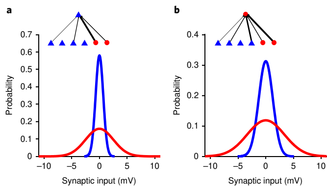
Fig. 4 | Synaptic rewiring in a feedforward network. a, b , The distributions of changes in time-averaged inputs to an excitatory ( a ) and an inhibitory ( b ) neuron in a feedforward configuration, following excitatory (blue) or inhibitory (red) rewiring. The wider the distribution, the larger the effect of rewiring is. For both the excitatory and inhibitory neurons, inhibitory rewiring has a larger effect than excitatory rewiring on the input to neuron.
