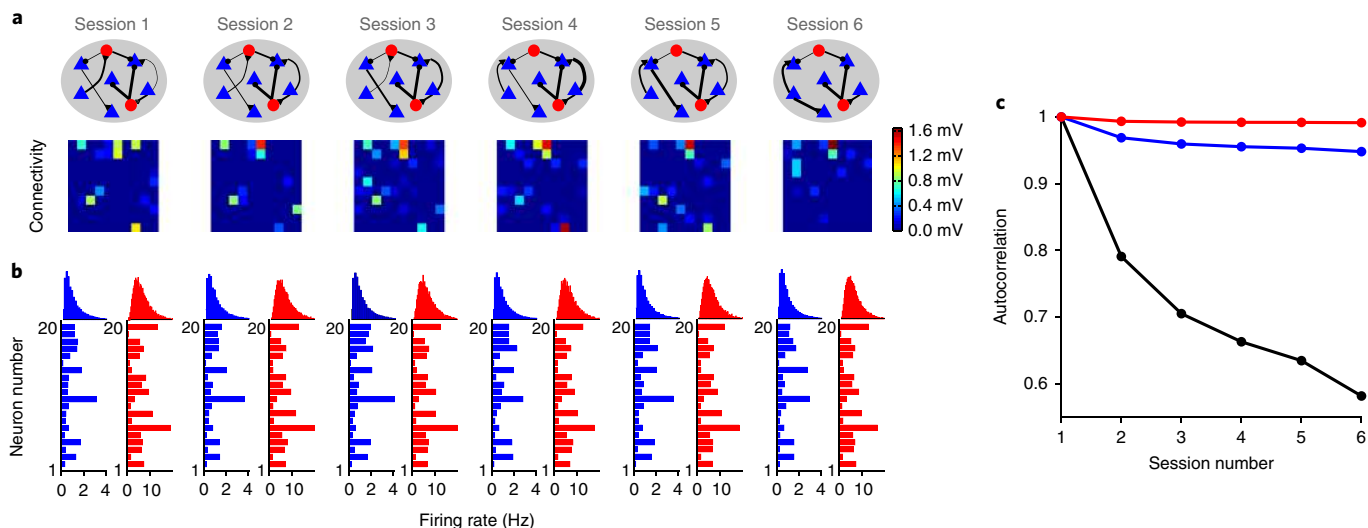
Fig. 2 | Volatility in the E \rightarrow E connectivity has little effect on network activity. a , Top: schematic illustration of six networks, each corresponding to the cortical network in one of the imaging sessions. Bottom: the connectivity matrix between ten randomly selected excitatory neurons. Color denotes the synaptic efficacy (deep blue, unconnected pair). b , Top: distributions of firing rates of the excitatory (blue) and inhibitory (red) neurons (session 1 is same as Fig. 1c). Bottom: the firing rates of 20 excitatory (blue) and 20 inhibitory (red) randomly selected neurons. c , Autocorrelograms of the E \rightarrow E connectivity matrices (black) and firing-rate vectors of the excitatory (blue) and inhibitory (red) neurons.
