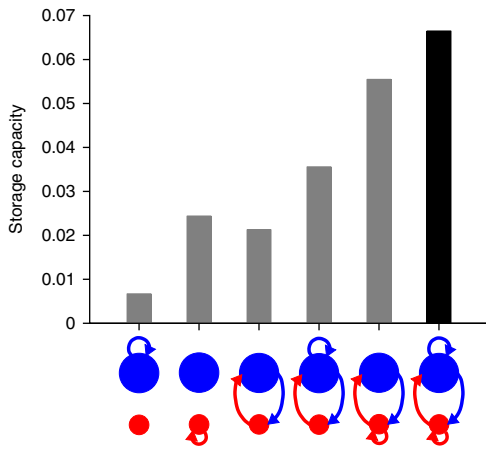
Fig. 6 | Storage capacity using different synaptic types. The memory capacity of a network is defined as the number of memories that the network can maintain relative to the total number of neurons in the network. We used mean-field approximation (see Methods) to estimate the memory capacity for random binary memory patterns (sparseness: 0.1). We used Hebbian and anti-Hebbian learning rules on the excitatory and inhibitory synapses, respectively, preserving the probabilities of connections and the marginal distributions of synaptic efficacies of Fig. 1a (see text and Methods). Bars depict the capacity when learning is restricted to different subsets of synapses. From left to right: E \rightarrow E ; I \rightarrow I ; E \rightarrow I & I \rightarrow E ; E \rightarrow E , E \rightarrow I & I \rightarrow E ; I \rightarrow I , E \rightarrow I & I \rightarrow E ; all synapses (black). Note that memory capacity when learning is restricted to E \rightarrow E synapses is less than one-third of the capacity when it is restricted to I \rightarrow I synapses. This is despite the fact that there are 8 times more E \rightarrow E synapses than I \rightarrow I synapses in the network. When learning is restricted to E \rightarrow E & I \rightarrow I synapses, the memory states of the inhibitory and excitatory parts of the network are dissociated (not shown).
