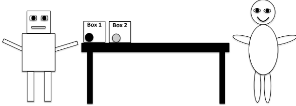
Figure 2: Balls in the boxes scenario
