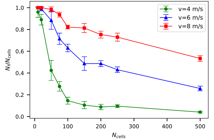
Fig. 6. Effect of the number of cells on the number of generated fragments for three different values of the impact velocity.
