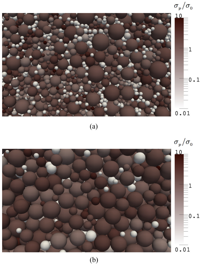
FIG. 17. Snapshots of samples with particles colored according to applied total stress \sigma_p on each particle normalized by the mean packing stress \sigma_0 both figures for \alpha = 5 . (a) Packing S5 with C_u = 2.43 and (b) packing S8 with C_u = 1.58 .
