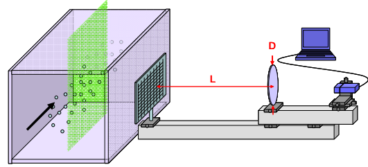
Figure 24: calibration procedure.
