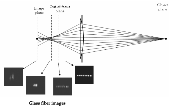
Figure 18 : Spherical aberration
