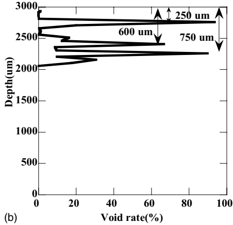
FIG. 7. (a) Image by SEM of a cross section of 3000 \mu\text{m} basalt foil at laser power density of 1.27 \pm 0.13 \text{ GW/cm}^2 ; (b) corresponding rate of void, calculated using SHYLAC software at time of 700 ns from the irradiation of 1.27 \pm 0.13 \text{ GW/cm}^2 (peak pressure loading: 1.7 GPa). Laser beam comes from bottom (location: 0 \mu\text{m} ). Rear free surface is on the top.
