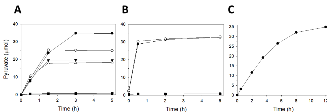
Figure 8. Optimization of the KG/PEP ratio in different KG phosphorylation reactions with ATP regeneration. (A) Reactions were performed in 1 mL of Tris-HCl buffer 50 mM and 50 \mu\text{mol} of the limiting substrate at different ratios of KG/PEP (1.0/0.5 (●), 1.0/0.7 (○), and 1.0/0.9 (▼), 1.0/1.1 (Δ)) and a control reaction with no ATP (■). (B) Reactions were performed in 2 mL of Tris-HCl buffer 50 mM and 40 \mu\text{mol} of the limiting substrate at different ratios of KG/PEP (1.0/0.5 (●) and 1.0/0.7 (○)) and a control reaction with no ATP (■). (C) Reactions were performed in 2.5 mL of Tris-HCl buffer 50 mM and 35 \mu\text{mol} of the limiting substrate employing a KG/PEP ratio of 1.0/0.8.
