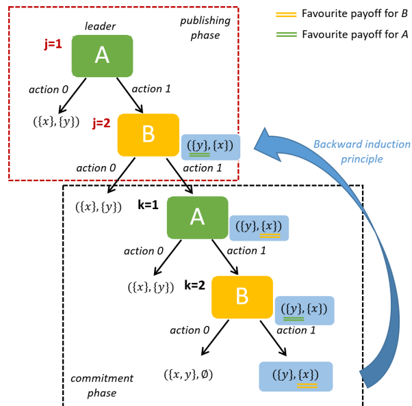
Fig. 3. Extensive form game associated to the blockchains swap protocol, presented in [16]. Publishing and commitment phases are sequentially executed one after the other. Outcomes represent the payoffs (assets) owned by Alice and Bob respectively. The figure represents the backward induction process for each decision step.
