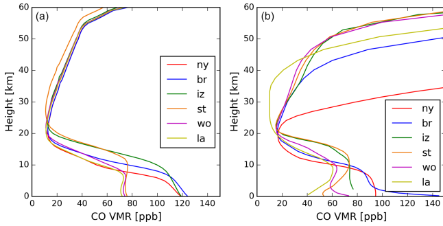
Figure 3. The CO a priori VMR profiles for TCCON (a) and NDACC (b) at six sites (ny: Ny-Ålesund; br: Bremen; iz: Izaña; st: Saint-Denis; wo: Wollongong; la: Lauder). As TCCON a priori profiles change every day, the mean profiles in 2013 are shown here.
