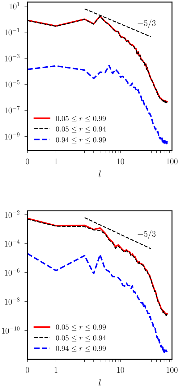
Figure 5. Power spectrum of the time-averaged and radially-integrated quantity -1/(\Delta T(\omega_t \beta)^2) \int \mathbf{u} \cdot [\mathbf{u} \cdot \nabla \mathbf{U}_0] dt , as a function of the spherical harmonic degree l \geq 0 (using orthonormalized harmonics). Simulations at Ra = 10^6, Pr = 1 and \beta = 5 \times 10^{-2} . Eddy viscosity (2) is given by the square-root of the l = 0 component (in the physical space), when \Delta T is large enough to reduce the turbulent noise. Top : |\omega_t|/\omega_{cv} = 2.3 with an integration time \Delta T \simeq 0.59 . Bottom : |\omega_t|/\omega_{cv} = 13 with an integration time \Delta T \simeq 0.39 . Spectra have been computed by interpolating the data to a spherical grid.
