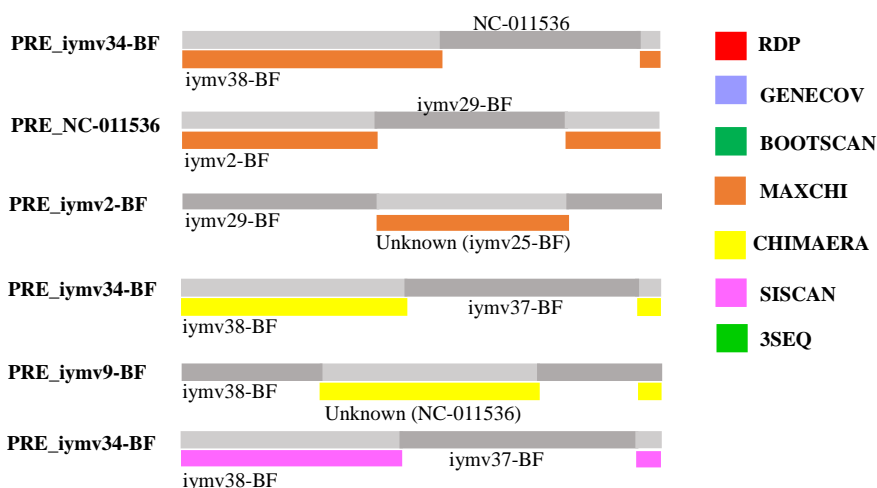
Figure 4. Description of potential recombination events. PRE_ymv34-BF, PRE_NC-011536, PRE_ymv2-BF and PRE_ymv9-BF are the Potential Recombinant Events (PREs). See text for details of major and minor parents.
