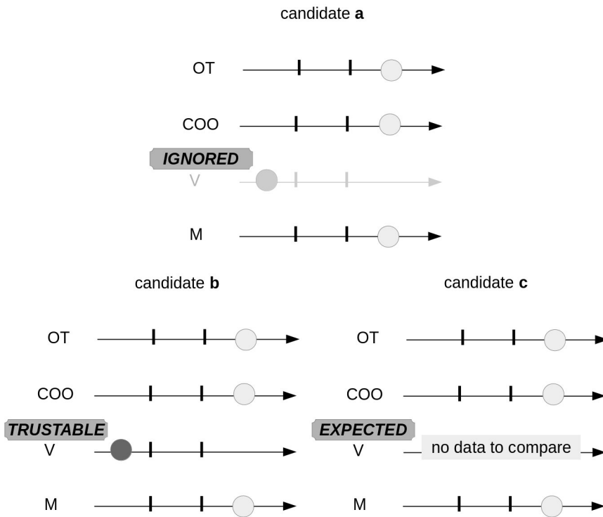
Figure 4. Examples of candidate evaluation with options: candidate which is labeled "good" (a); candidates which are labeled "bad" (b, c).
