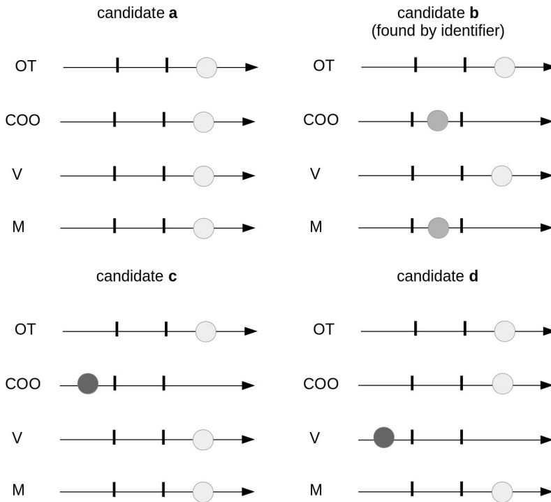
Figure 3. Examples of candidate evaluation by default: candidates which are labeled "good" (a, b); candidate which is labeled "bad" (c); candidate which is labeled "undefined" (d).
