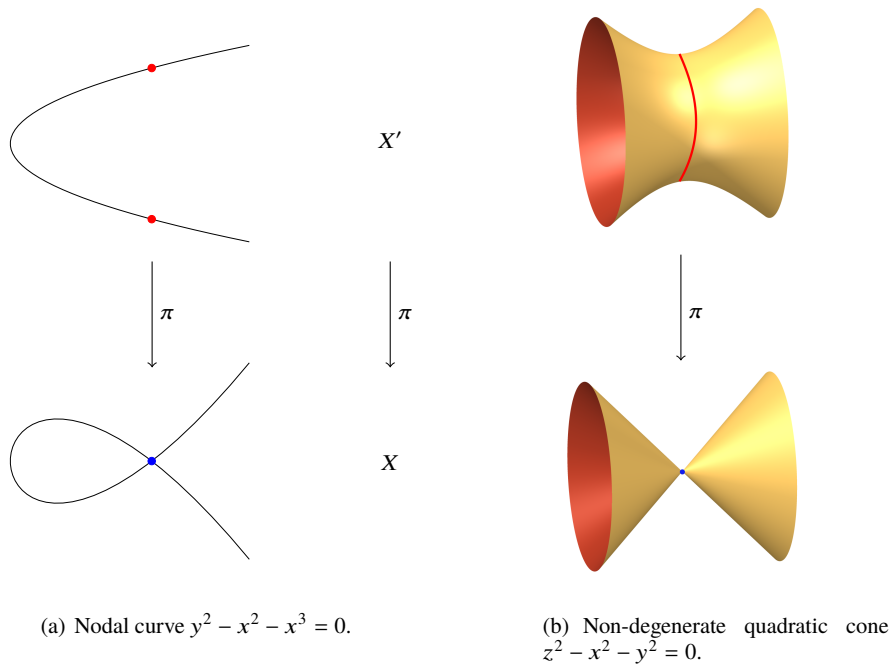
Fig. 1.1 Resolution of singularities. The center of the blowing up is in blue and the exceptional set in red.
