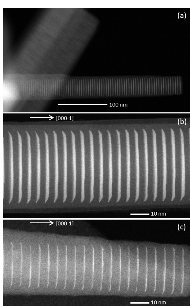
Figure 3. (a) HAADF-STEM image of dispersed NWs containing 88 periods of GaN/AlN (1.5 nm/3.0 nm). The bright contrast is GaN and the darker contrast represents AlN. Note that in HAADF-STEM the contrast of the image provides chemical information. (b) High-magnification HAADF-STEM image of a NW containing 88 periods of GaN/AlN (S1). (c) High-magnification HAADF-STEM image of a NW containing 88 periods of Al 0.1 Ga 0.9 N/AlN (S5).
