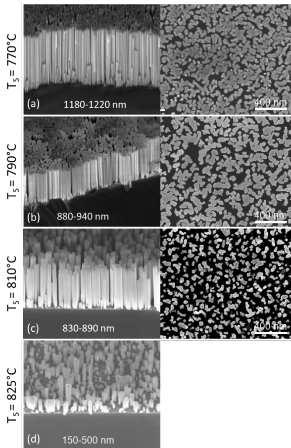
Figure 1. SEM images (bird's eye on the left and top view on the right side) of GaN NW samples grown at various substrates temperatures: (a) 770^\circ\text{C} , (b) 790^\circ\text{C} , (c) 810^\circ\text{C} , and 825^\circ\text{C} . The NW height is indicated as a legend in the bird's eye figure. All the samples grew for 3 hours with a flux ratio \Phi_{\text{Ga}}/\Phi_{\text{N}} = 0.25 .
