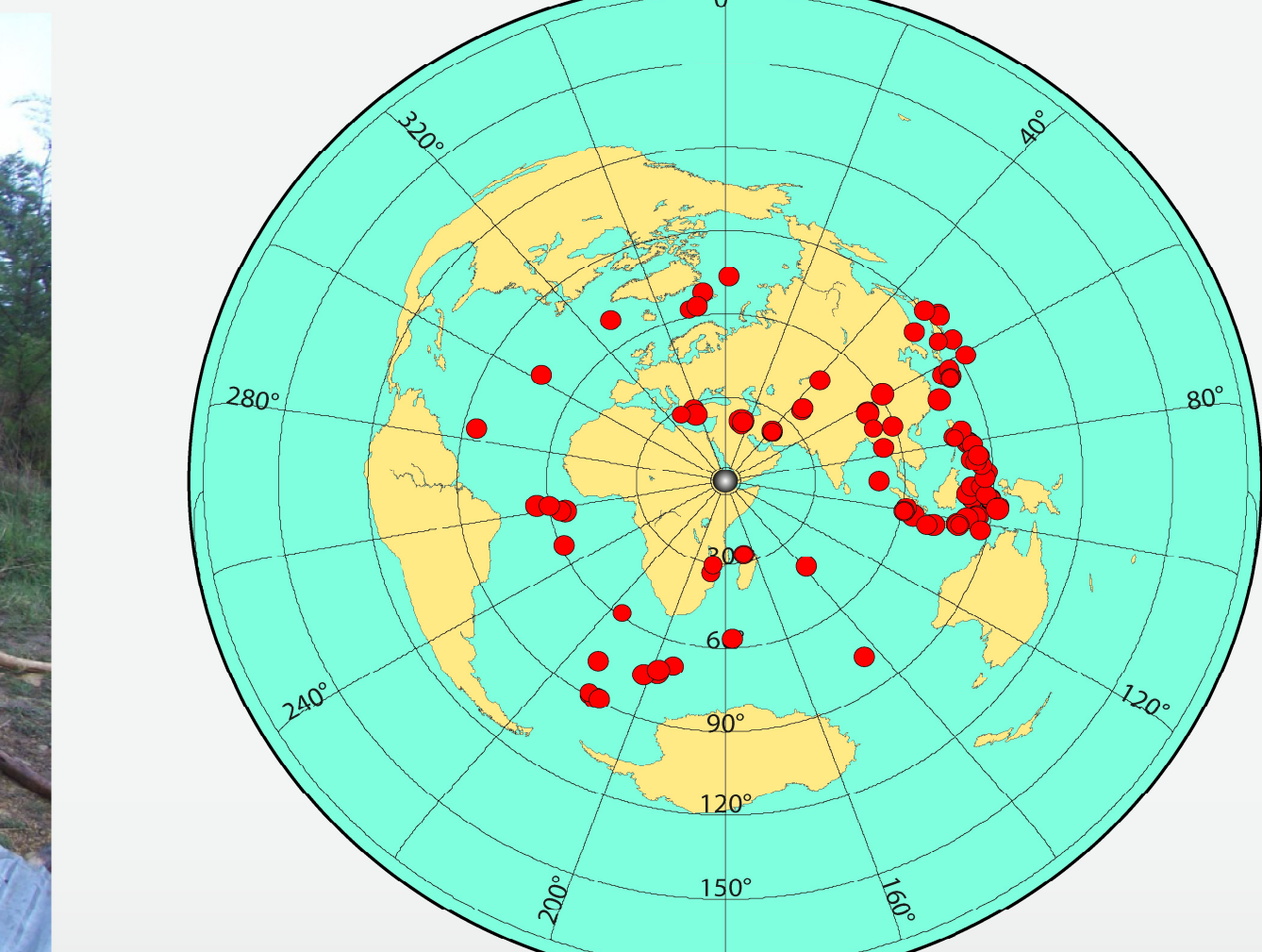
Fig.(4) map showing the distribution of the teleseismic events used in this study centered at the network location.
