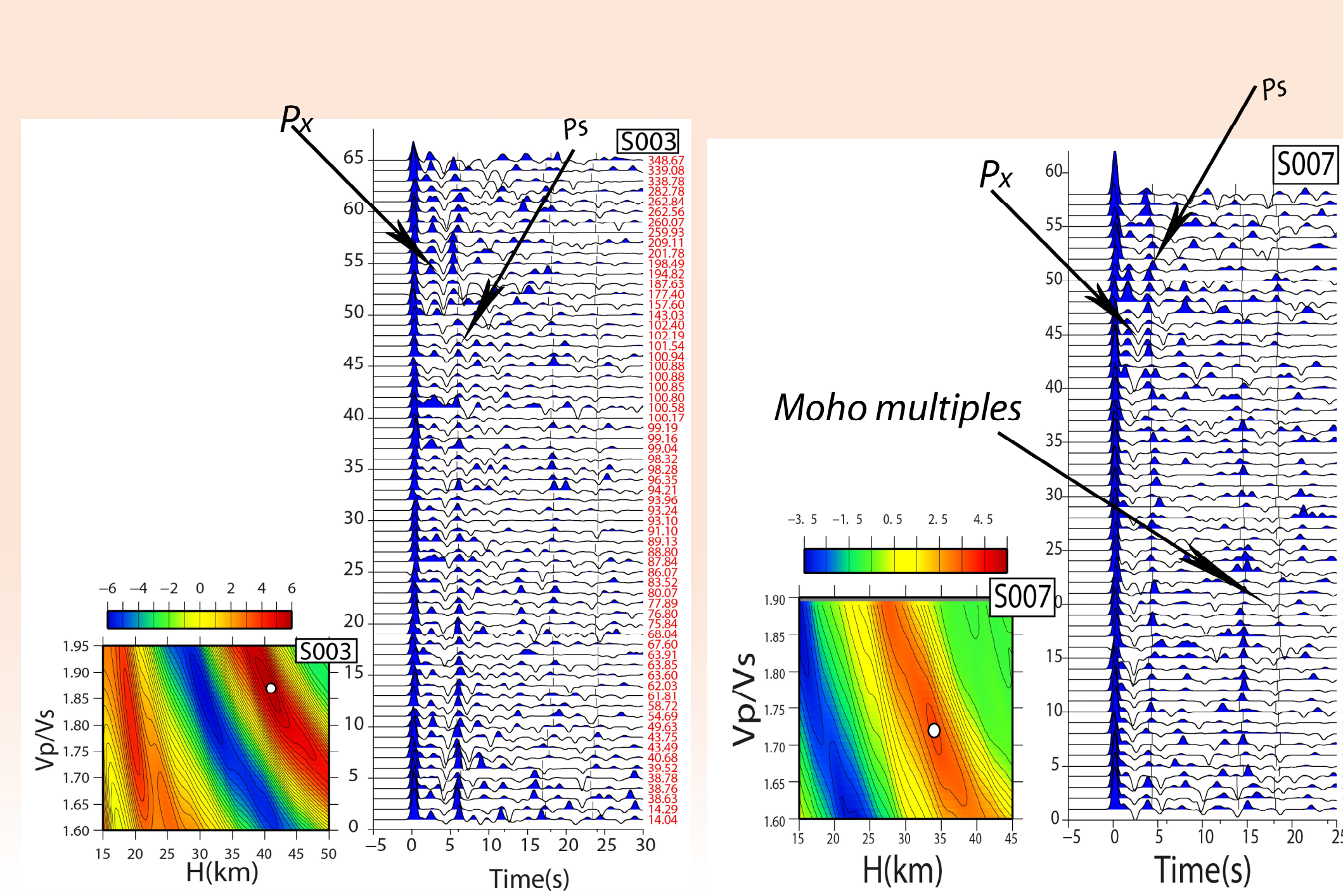
Fig.(6) Some of the RF results from the southern profile:
