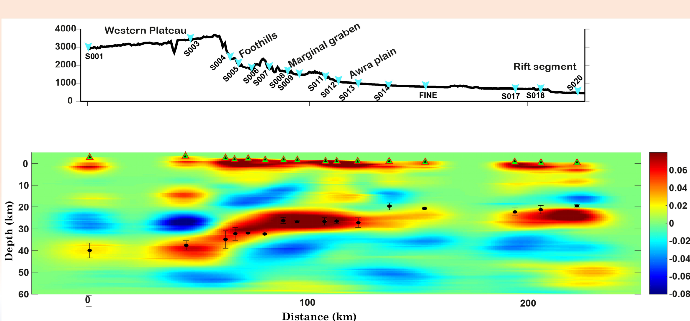
Fig.(11) The CCP migrated cross section along the southern profile: - The Moho depth is in the range ~ 40-19.0 km. - We estimate the crust thinning occurs in 4 steps along the profile between the stations S003-S005, S007-S008 and S013-S014. - These 4 steps divided the area between the western plateau and the rift axis to four distinct regions of uniform crustal thickness. - A clear intra-crustal interface could be seen along the profile.
