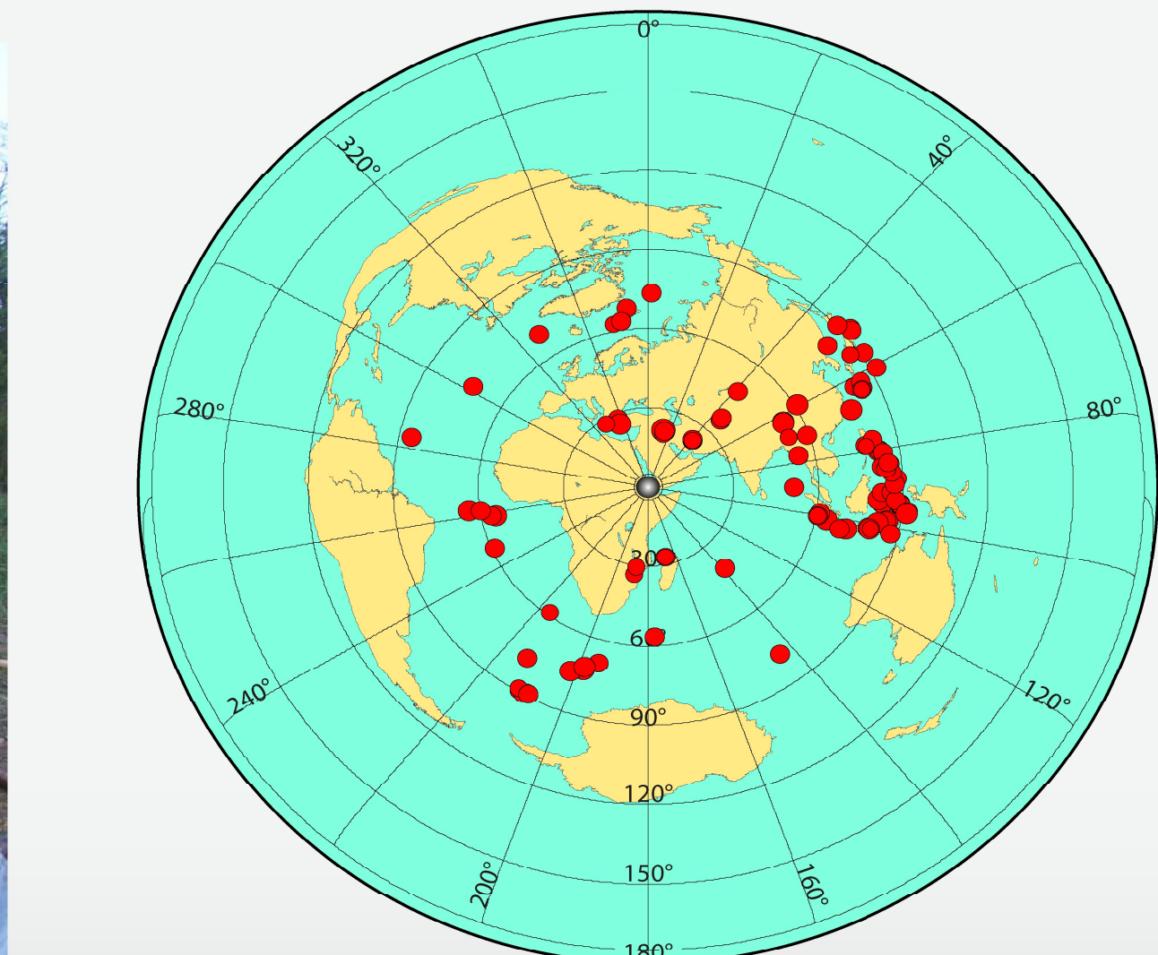
Fig.(4) map showing the distribution of the teleseismic events used in this study centered at the network location.
