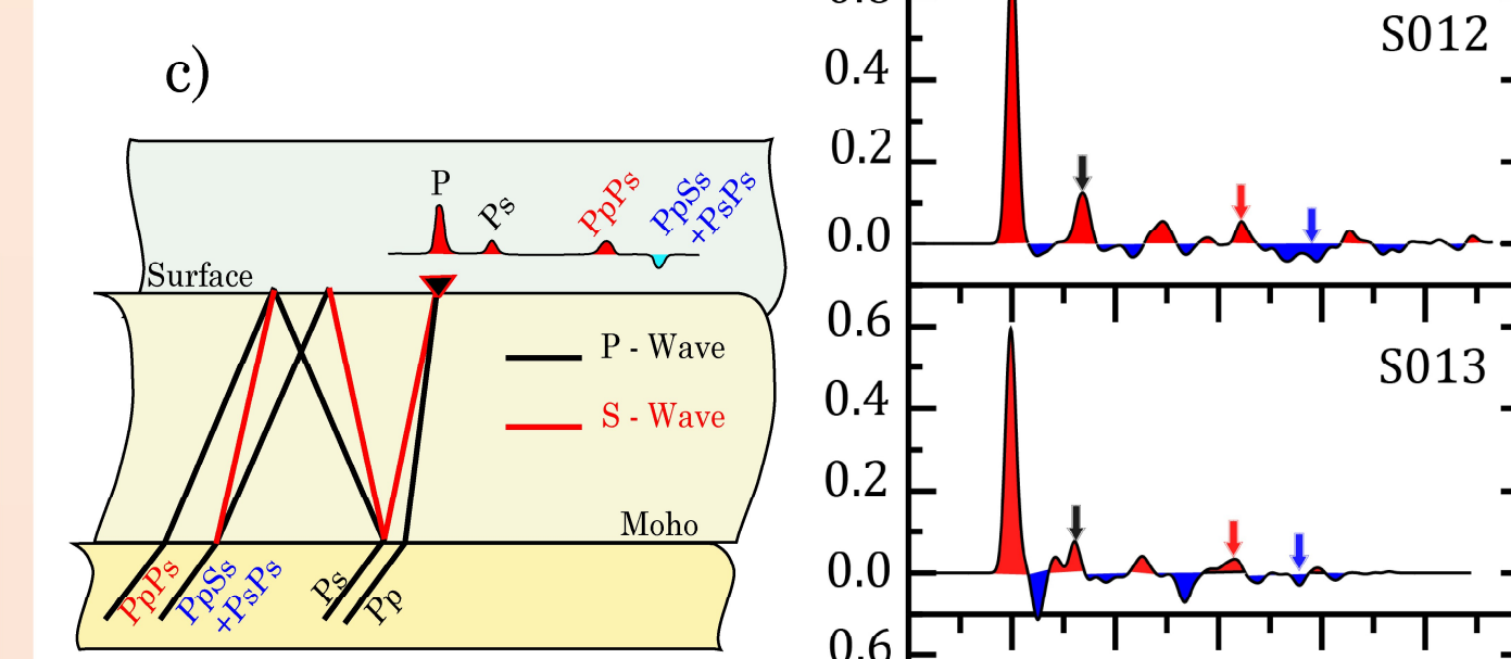
Fig.(7) Stacked receiver functions for the seismic stations along the two profiles. a) the northern profile - Danakil Depression, b) the southern profile at the latitude of the central Afar, and c) sketch illustrating the path of the converted phases and
