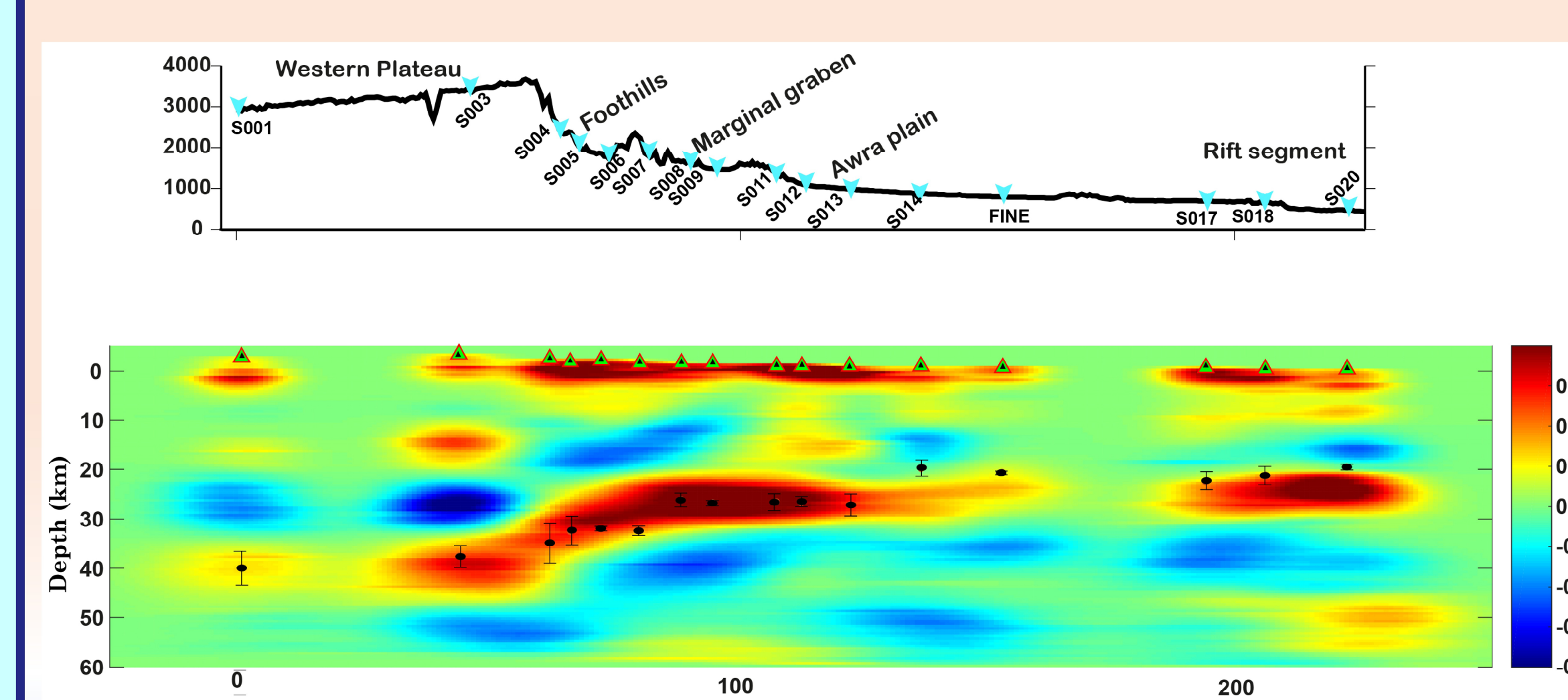
Fig.(11) The CCP migrated cross section along the southern profile: - The Moho depth is in the range ~ 40-19.0 km. - We estimate the crust thinning occurs in 4 steps along the profile between the stations S003-S005, S007-S008 and S013-S014. - These 4 steps divided the area between the western plateau and the rift axis to four distinct regions of uniform crustal thickness. - A clear intra-crustal interface could be seen along the profile.
