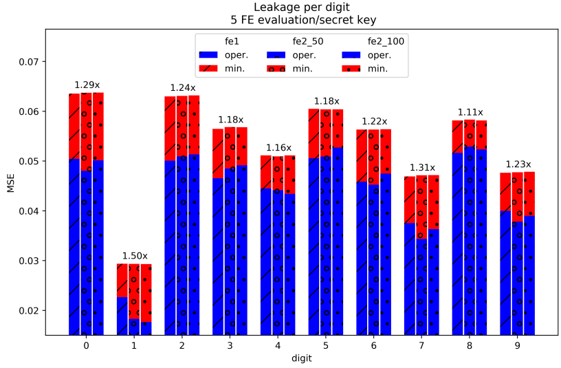
Fig. 6. MNIST – per digit information leakage estimation.
