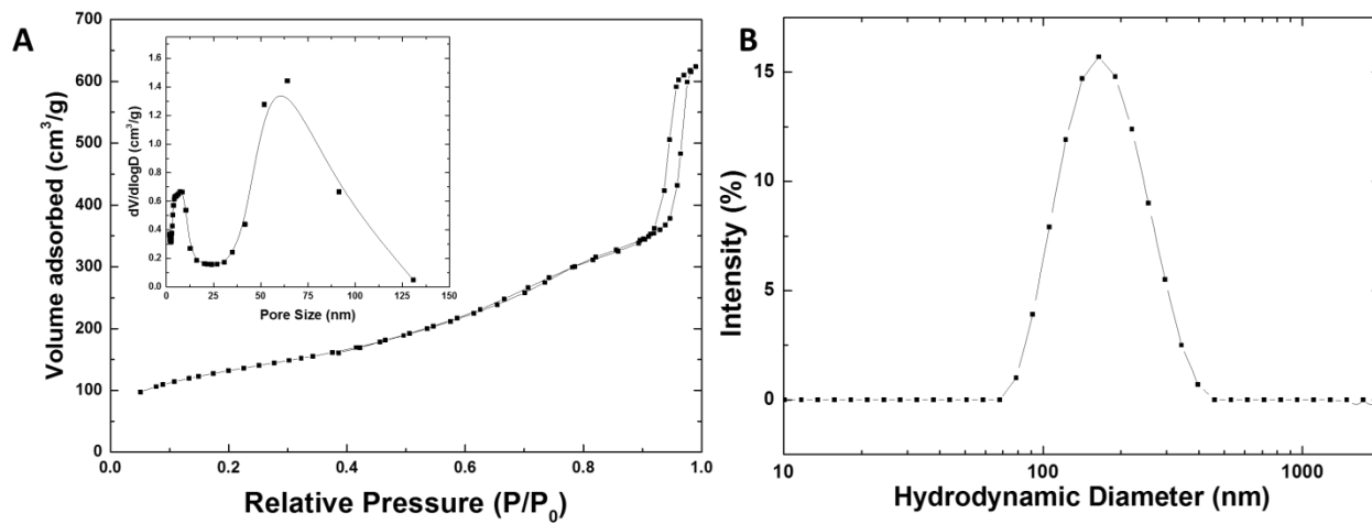
Figure S3. (A) N 2 physisorption isotherms of IO@STMSNPs and the corresponding pore size distribution curve in inset calculated by the BJH method. (B) DLS size distribution (intensity) of IO@STMS NPs dispersed in water (pH=7).
