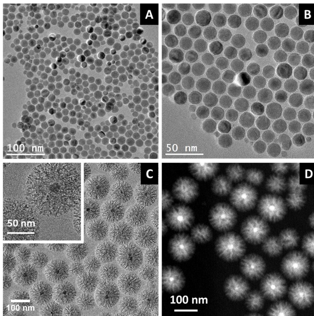
Figure 2. TEM images of 18 nm size IO spherical NPs over (A) a large zone and (B) at a higher magnification. (C) TEM image of stellate porous core shell IO@STMS NPs. The inset shows an image at higher magnification. (D) STEM-ADF image of stellate porous core shell IO@STMS NPs.
