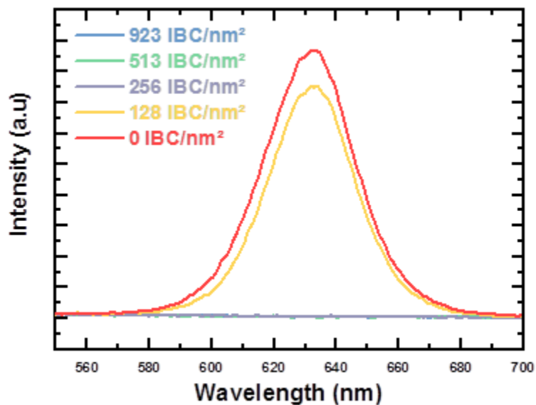
Figure S5. Fluorescence emission intensity of IBAM-modified IO@STMS@QDs nanocomposites in the following conditions = 923, 513, 256, 128, IBC.nm -2 and without IBC.
