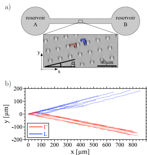
Fig. 16 a) Schematic top-view ( x - y plane) of the microfluidic channel containing a periodic post array, inclined by an angle \alpha with respect to the channel axis ( x -direction). Fluid and particles can be injected into the linear channel via two reservoirs at its ends. A steady fluid flow through the channel is generated by a pressure difference applied to the two reservoirs. The magnified inset shows an optical micrograph image of the square lattice of cylindrical posts, as well as two L-shaped particles of opposite chirality coloured in blue (L particle) and red (R particle). b) Experimental trajectories observed in the set-up from (a) with \alpha=15^\circ for several of the both chiral particles from (a), demonstrating chiral separation in the post array. Adapted from Ref. 47 with permission from the American Physical Society
