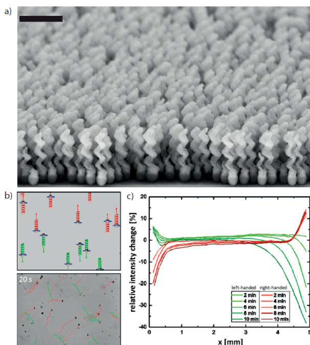
Fig. 9 The propeller effect at the colloidal scale. a) SEM images of a wafer containing helices representative of those used in Ref. 26 obtained through glancing angle deposition. Scale bar is 2 μm. b) When a field is applied, the magnetic moments of the helices (perpendicular to their long axis) aligns with the field direction and rotates with it. The rotational-to-translational coupling then allows right- and left-handed helices to move in opposite directions. c) Relative intensity change with time of the scattering intensity across the width of a 5 mm cuvette filled with a suspension of right- or left-handed colloids in a rotating magnetic field of a strength of 50 Gauss and a frequency of 40 Hz. Adapted from Ref. 26 with permission from the American Chemical Society.
