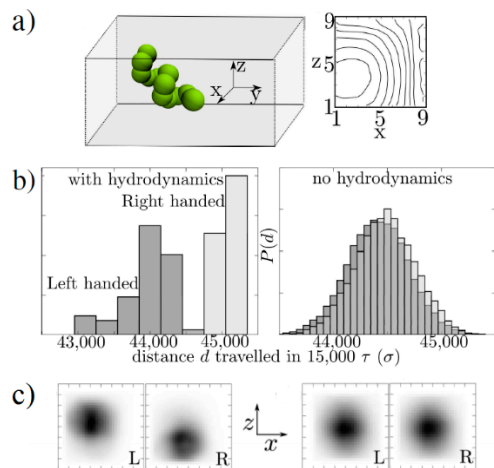
Fig. 13 a) Illustration of the set-up simulated by Meinhardt 39 using dissipative particle dynamics. The chiral helical particle (green object) is advected along the y-direction through a microchannel (grey rectangular box) with square cross-section (x-z plane) by a pressure-driven fluid flow, which is asymmetric due to different hydrodynamic boundary conditions on the four channel walls. The right panel shows profiles of equal flow velocities across the channel. b) Separation of right-handed and left-handed helical particles. Histograms of distances travelled along the channel axis (y-direction) in a certain time for left-handed helices (dark shaded) and right-handed helices (light shaded) are shown. Results from simulations, which take full account of hydrodynamic effects (left part), are compared to a simple Brownian dynamics simulation without hydrodynamics (right part). c) Distributions for left-handed (L) and right-handed (R) helices across the channel in the two cases with and without hydrodynamics. The quantities \sigma and \tau represent the basic length and time-units in the simulation model. Adapted from Ref. 39 with permission from the American Physical Society.
