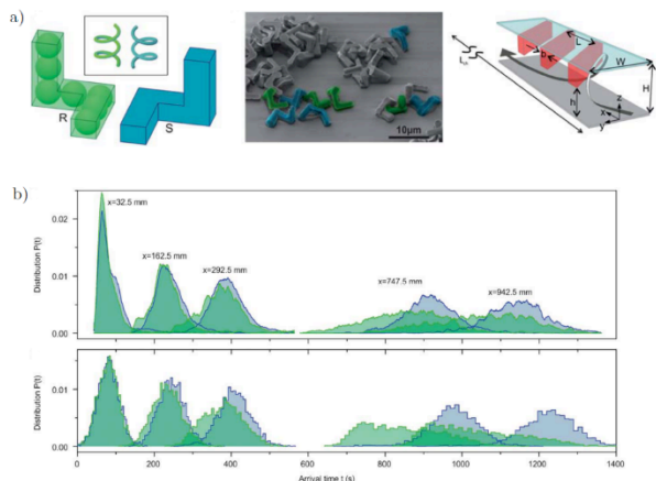
Fig. 14 a) Experimental set-up used by Aristov et al. 41 The left panel shows the schematic illustration of particles of opposite chirality R (green) and S (blue). They consist of three mutually perpendicular “legs” of equal length (about 6 \mu\text{m} ) as simplified representations of real helices. In the theoretical model, the chiral colloids have been represented by 7 rigidly connected beads. The middle panel shows a false-coloured SEM micrograph. The right panel shows a schematic of the microfluidic channel (side walls not shown) with periodically arranged oblique ridges (red) which create a swirling flow pattern ( W=150 \mu\text{m} , H=115 \mu\text{m} , H-h=50 \mu\text{m} , b=40 \mu\text{m} , L=146 \mu\text{m} , and L_{\text{ch}}=1 \text{ m} ). (b) Arrival time distributions at various fixed positions x along the channel axis from experiments (upper panel) and simulations (lower panel) demonstrating separation of the chiral colloidal particles in a right-handed helical flow field. Adapted from Ref. 41 with permission from the Royal Society of Chemistry.
