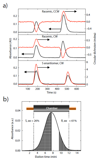
Fig. 11 Enantioenrichment of a racemic mixture of the 1,1'-Bi-2-naphthol bis(trifluoromethanesulfonate) molecules after 83 hours of REF. a) (Top) Absorbance and Circular Dichroism chromatograms of a racemic mixture while turning the field CCW (middle) CW and (bottom) CW for the pure S enantiomer. One can see on the chromatograms that the leading and the trailing fractions of the chamber display opposite CD signals that is reversed when the rotation direction of the field is reversed. (Bottom) When a pure S enantiomer is loaded in the cell and submitted to the same experimental condition, both fractions display a CD signal of the same sign which is a control experiment for chiral migration observed in the previous racemic experiments. b) Absorption chromatogram of the chambers slug after being exposed a CW REF collected from the in-line detector. The slug can be decomposed in two halves (grey areas). The first left half was enriched with the (S)-1,1'-Bi-2-naphthol bis (trifluoromethanesulfonate) whereas the second one was enriched with the R-analogue by 61 percent. Adapted from Ref. 27 with permission from the Royal Society of Chemistry.
