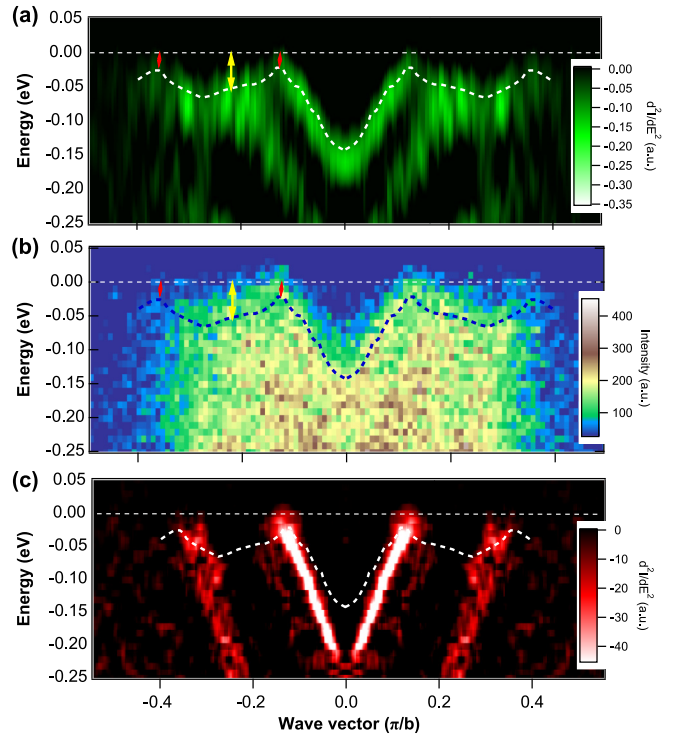
FIG. 9. (a) Second derivative (with respect to energy) of the ARPES intensity measured with s polarization. (b) Corresponding raw data measured in s polarization. Both (a) and (b) evidence the backfolding resulting from the hybridization of bands A1^+ , A2^+ , and C2. The gap amplitudes (arrows) can be estimated from the distance between the E_F and the edge profile. (c) Second derivative with respect to energy of the ARPES intensity measured with p polarization. The spectral intensity exhibits a gapless behavior and a linear dispersion with no backfolding evidences. The dashed wriggling line shown on each panel follows the inflection point of the spectral intensity at the vicinity of E_F in the s polarization.
