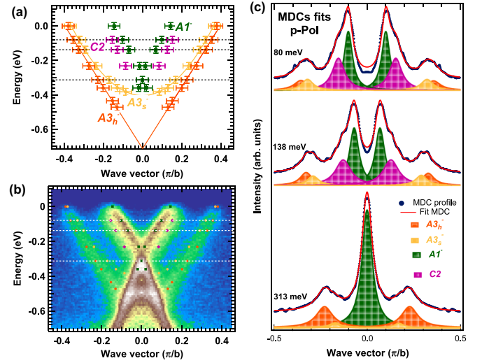
FIG. 12. (a) Band dispersion obtained from MDCs fits for p polarization. (b) Results of the MDCs fit superimposed on the ARPES intensity image. The dashed lines indicates the energy profiles for MDCs shown in (c). Dark and light orange features display the double structure composing band A3^- related to possible spinon and holon contributions.
