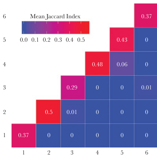
Figure 2 Cluster matrix of Mean Jaccard Index between monthly home range of female chamois.
