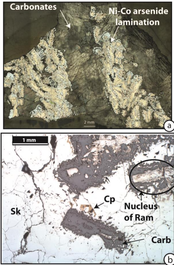
Figure 2. a. The “ contact ” type composed of laminated contact mineralization (LCM) of Ni-Co rich arsenide then surrounding by carbonate (image in reflected light). b. Nucleus of Rammelsbergite surrounding by skutterudite, carbonate, chalcopyrite, in a massive gangue of skutterudite and carbonates, indicates a brecciated-related environment of the contact mineralization (BRCM) (image in reflected light). Carb: carbonate, Co: Cobalt, Cp: Chalcopyrite, Ni: Nickel, Ram: Rammelsbergite, Sk: skutterudite
