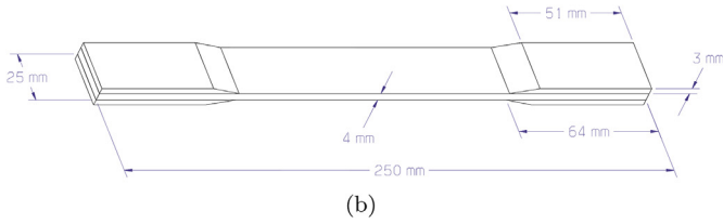
Fig. 3. (a) Hot platen press consolidation setup for composite plate manufacture, [0/90]_{45} layup is shown as an example only; (b) Test specimen dimensions.
