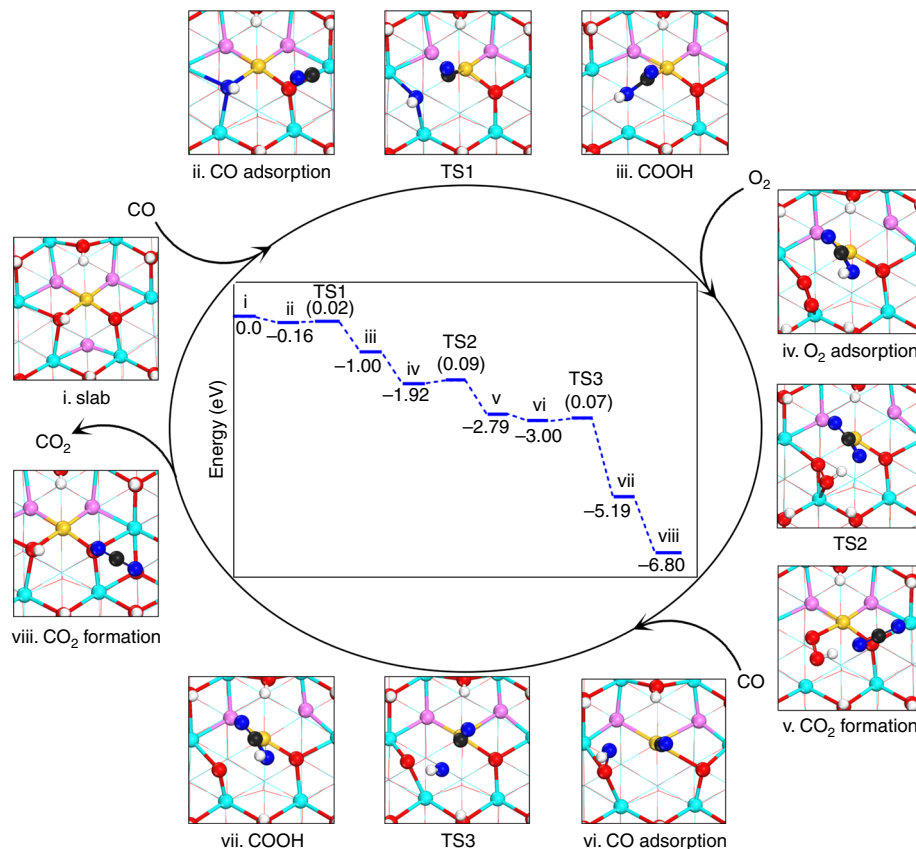
Fig. 3 Reaction pathway B for CO oxidation on the Au 1 /CeO 2 (111). The inset (within the ellipse) shows the potential energy profile and the numbers in the parentheses indicate the barriers (in eV) of elementary steps
