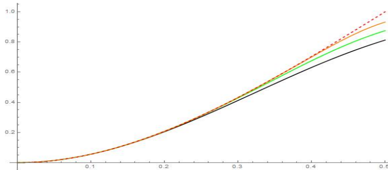
FIGURE 1. Graph of q \mapsto P_A(2) , A = 3, 5, 10 and asymptotics A \rightarrow +\infty
