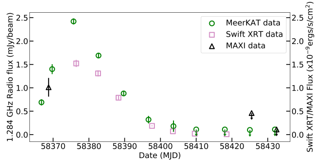
Figure 1. The radio (green circles), Swift X-ray (pink squares) and MAXI (black triangles) light curves of the 2018 Outburst of H1743–322, from the data in Section 2.2 and shown in Table 1. The upper limits are denoted with downward arrows in the MeerKAT and MAXI data. The X-ray data are obtained from fitting MAXI or Swift XRT data in the unabsorbed 1–10 keV energy range. The radio and X-ray data roughly track with each other, as expected given the radio/X-ray correlation in BHXBs.
