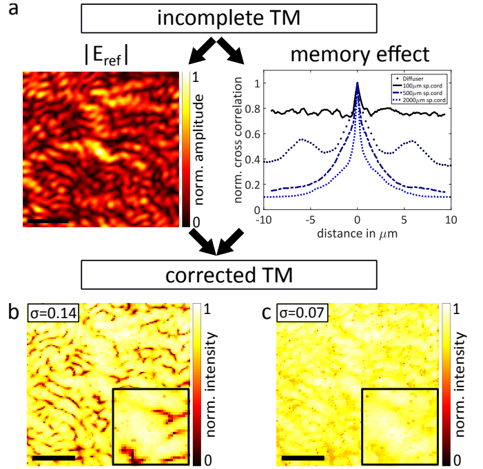
Fig. 2. a) Schematic principle of the TM correction based on the memory effect. The reference field amplitude and the memory effect are extracted from a TM measurement. The memory effect is represented for different samples (see text). b) Refocus intensity scans obtained with the uncorrected TM through a 500 \mu\text{m} thick mouse spinal cord tissue. c) Similar scan with the corrected TM. \sigma : standard deviation of the image intensity. Scale bar: 5 \mu\text{m} .
