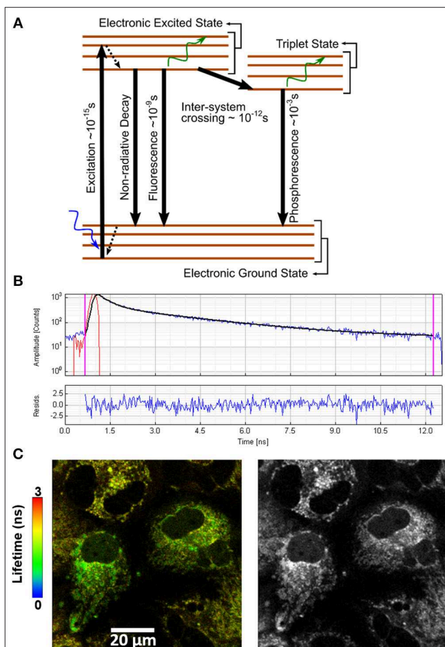
FIGURE 2 | (A) Energy band diagram. (B) Typical bi-exponential model fitting of NAD(P)H fluorescence decay curve. The standard-fitted fluorescence decay curve is shown with \chi^2 close to 1 and residuals showing no noticeable systematic variations. The y-axis is in photon counts, and x-axis is the time in nanoseconds. (C) NAD(P)H representative color-coded image of NAD(P)H lifetimes (left) and fluorescence intensity (right) in Huh 7 cells. Figure reproduced (from [50]) with kind permission from Springer.
