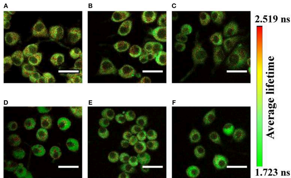
FIGURE 3 | Shows the autofluorescence lifetime images of NADH by pseudocolor mapping in PC12 cells (A) differentiated and untreated; and treated with (B) 50, (C) 100, (D) 250, (E) 500, and (F) 1,000 \mu\text{M} of MPP + . The color bar represents the range of the average fluorescence lifetime. Figure reproduced (from [33]) with kind permission from Springer Nature. Scale bar: 20 \mu\text{m} .
