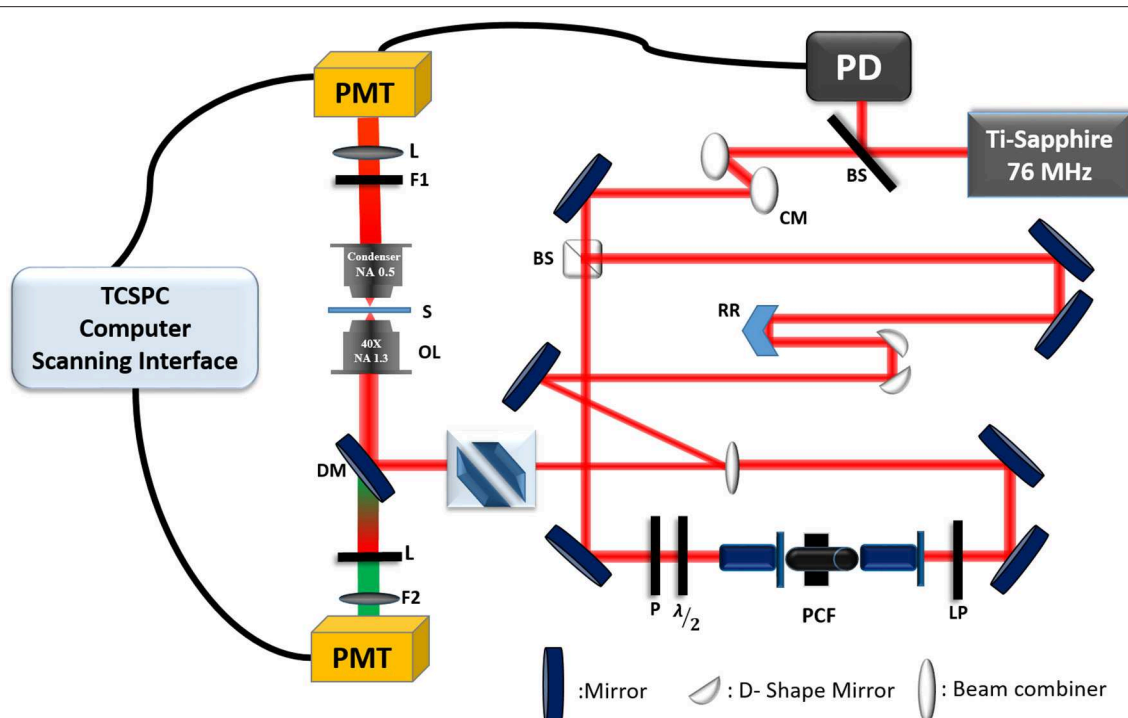
FIGURE 10 | Experimental setup of CARS microscopy integrated into a time-resolved fluorescence lifetime imaging system. BS, beam splitter; PD, photodiode; CM, chiral mirror; RR, retro-reflector; LP, long-pass filter; PCF, photonic crystal fiber; \lambda/2 , half-wave plate; P, polarizer; DM, dichroic mirror; OL, objective lens; S, sample; F1, 670/30 nm filter; L, lens; F2, 480/40 nm filter; PMT, photomultiplier tubes; TCSPC, time-correlated single-photon counting. The figure is reproduced with permission from Slepnev et al. [150, 151] and Pegoraro et al. [152].
