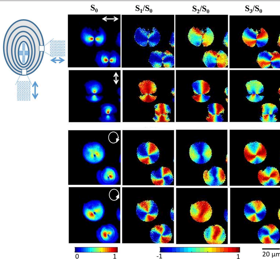
FIGURE 8 | Experimental reconstructed 2D Stokes images of the SHG response from starch granules for horizontally, vertically, right and left circularly polarized illumination, respectively. White arrows in the leftmost images indicate the direction of polarization. The color scale shows the value of each Stokes parameter increasing from blue to red. The figure has been reproduced with permission from OSA [111].
