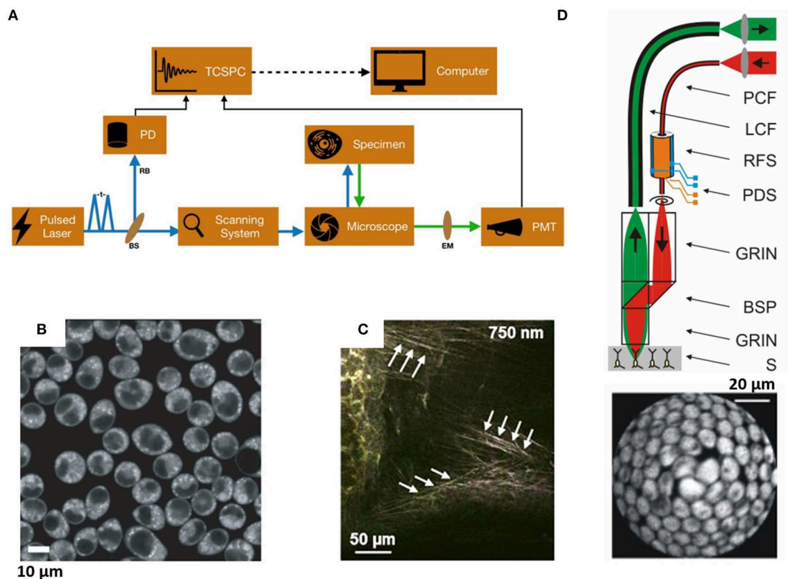
FIGURE 1 | (A) Typical schematic of two-photon fluorescence microscopy integrated with TCSPC system for fluorescence lifetime imaging: t, pulse interval; EM, emission filter; RB, reference beam; BS, beam splitter; TCSPC, time-correlated single-photon counter; PD, photodiode; PMT, photomultiplier tube [5]. (B,C) Two-photon auto-fluorescence images of (B) NAD(P)H in Rat basophilic leukemia (RBL) cells [6]; (C) Elastic fibers in the murine trachea ex vivo was detected between 400 and 580 nm at an excitation wavelength of 750 nm [7]. (D) Schematic of an ultra-compact fiber-optic two-photon fluorescence microscope. The near-IR ultrafast laser pulses (red) are passed through a hollow-core photonic crystal fiber to the microscope. The fluorescence emission (green) from sample (S) were guided through a large core fiber (LCF) and detected by a photomultiplier tube. The excitation and fluorescence signals were collected through custom-designed combination of GRIN lens and micro beamsplitter prisms (BSP). Two-photon fiberscope images of 10-micron diameter fluorescent microspheres were obtained by scanning spiral pattern trajectory for image reconstruction. PDS, piezo drive signals; RFS, resonant fiber scanner. Average laser power levels of 1 mW and 10x averaging were used. Scale bars are 20 \mu\text{m} [8]. All the Figures were reproduced with kind permission from respective publishers. The arrows indicate that those are elastin fibers.
