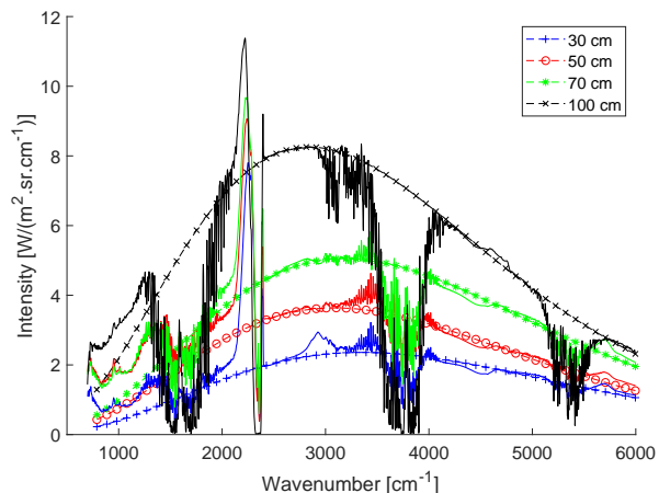
Figure 12: Mean emission spectra for fire width up to 100 cm, and the adjustments using the two-parameter model (i.e. Equation 7 with \alpha fixed).
