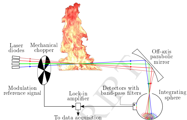
Figure 2: Elements of the opacimetry setup.
