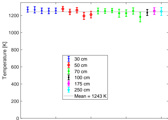
(b) Temperature T . The mean value (horizontal line) is based on all results.
