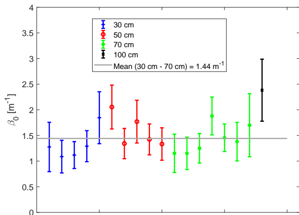
(a) Extinction coefficient \beta_0 . The mean value (horizontal line) is based on results for fire widths less than or equal to 70 cm.
