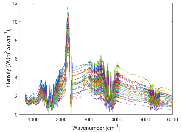
Figure 7: Examples of “instantaneous” spectra for a 50 cm wide flame.
