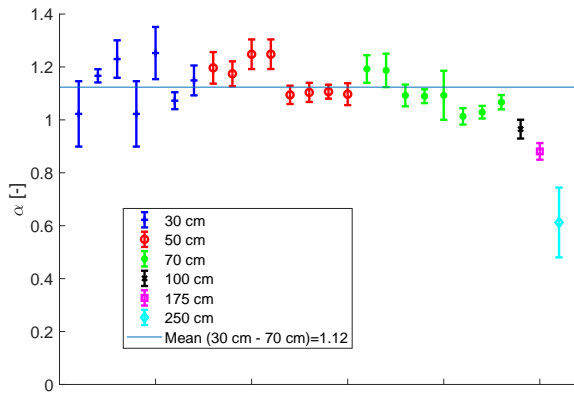
(b) Exponent \alpha .
