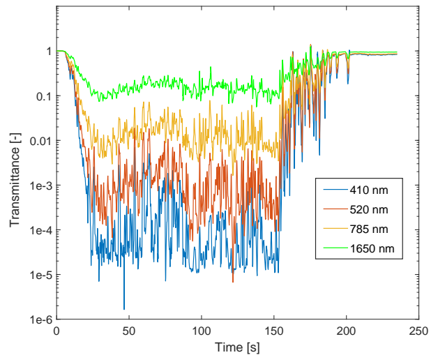
Figure 4: Spectral flame transmittance (log scale) for a 70 cm wide pan at four wavelengths in visible and near-infrared ranges.
