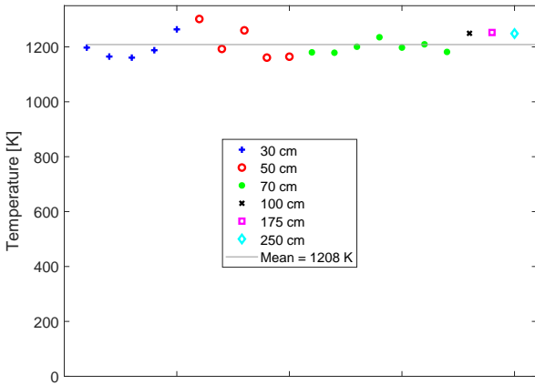
Figure 9: Identified temperatures from adjustments made on mean spectra using the one-parameter model (i.e. Equation 7 with \alpha and \beta_0 fixed).
