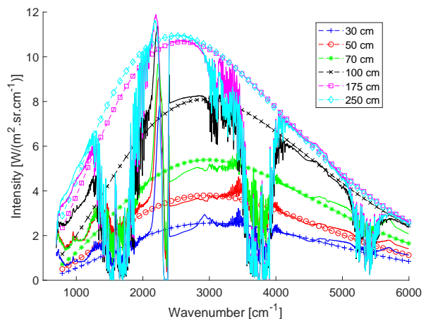
Figure 8: Mean emission spectra for all fire sizes, and the adjustments using the one-parameter model (i.e. Equation 7 with \alpha and \beta_0 fixed).
