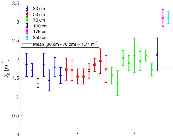
(a) Extinction coefficient \beta_0 .
