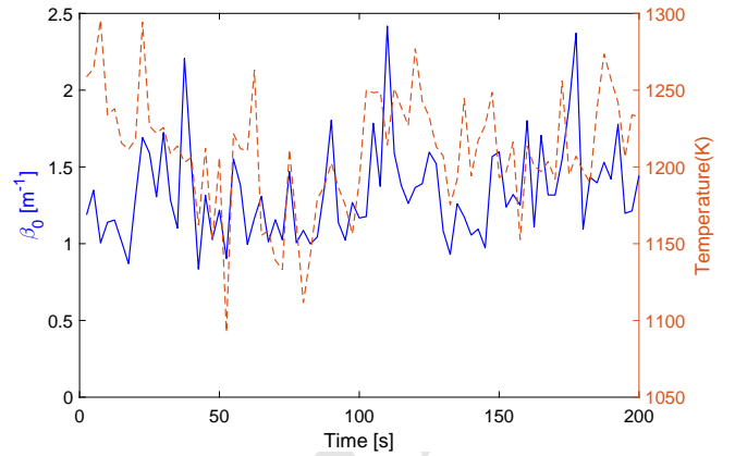
Figure 10: Temperature T and extinction coefficient \beta_0 identified from adjustments on “instantaneous” spectra using the two-parameter model (i.e. Equation 7 with \alpha fixed). Flame thickness equal to 50 cm.
