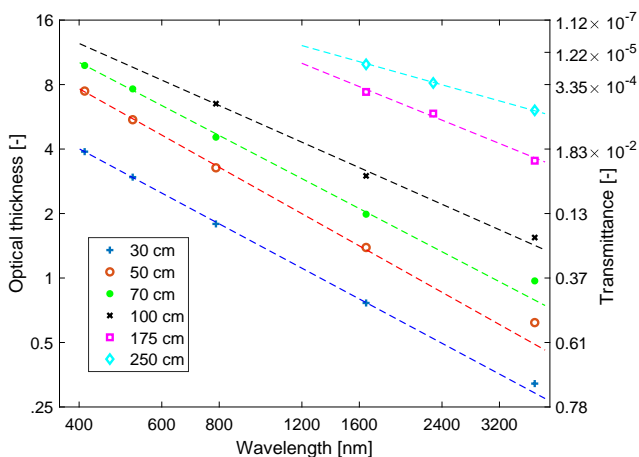
Figure 5: Mean optical thickness as a function of wavelength for various fire sizes, in log-log base 2 scale.
