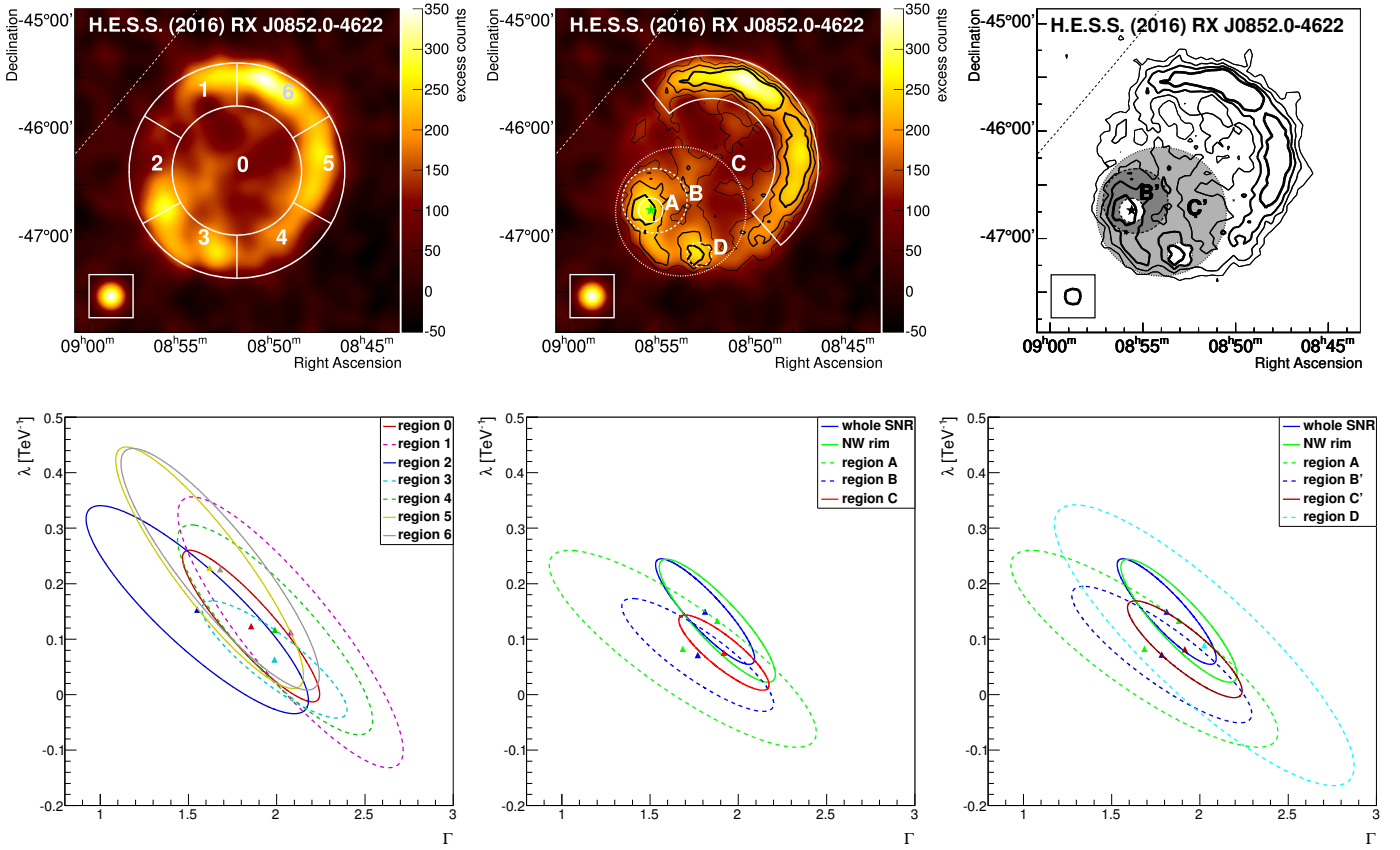
Fig. 4. Top figures represent skymaps (smoothed exposure-corrected excess map from Fig. 1 for the top left and center pads, significance contour map for the right pad) together with various regions used for the study of the spatially resolved spectroscopy of the RX J0852.0–4622 region. Top left: regions 0 for the central part of the SNR and 1–6 for the shell are shown in white. Center: regions A, B, and C around PSR J0855–4644, region D around the southern enhancement in the azimuthal profile, and the region used for the NW rim are shown in white. The H.E.S.S. significance contours at 5, 7, and 9 \sigma are shown in black with increasing line width for increasing significance. The position of PSR J0855–4644 is denoted by the green star. Top right: regions B' (dark gray shaded area) and C' (light gray shaded area) around PSR J0855–4644 are shown. The H.E.S.S. significance contours at 3, 5, 7, and 9 \sigma are shown in black with increasing line width for increasing significance. The position of PSR J0855–4644 is denoted by the black star. Bottom figures represent the error contour plots of \lambda = 1/E_{\text{cut}} vs. \Gamma for the spectra of the regions in the excess maps assuming a power law with exponential cutoff model. For each region, the fitted value is indicated with a triangle, while the ellipse indicates the contour of the 3 \sigma confidence level statistical uncertainty. Dashed lines are used for the regions where the cutoff significance is below 3 \sigma . Bottom left: spectra of the regions 0 to 6 are represented. Bottom center: spectra of the regions A, B, and C are represented. In addition, the contours of the analysis of the whole SNR and NW rim are shown. Since the spectra of regions A–C are correlated because the regions overlap, the corresponding contours are not meant to be compared to each other, but to the contours of the NW rim. Bottom right: spectra of the regions A, B', C', and D are represented. In addition, the contours of the analysis of the whole SNR and the NW rim are shown.
