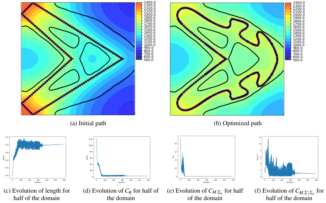
Figure 15: Initial and final temperature distribution and convergence histories, path optimization for the three holes cantilever from a hat initialization ( \eta = 5d_{lower} )
