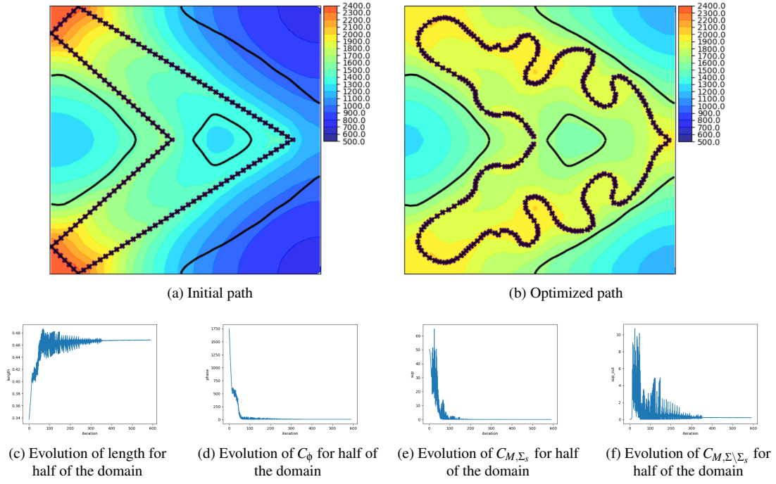
Figure 13: Initial and final temperature distribution as well as convergence histories, path optimization for the one hole cantilever from a contour initialization ( \eta = 5d_{lower} )
