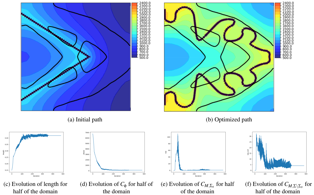
Figure 14: Initial and final temperature distribution as well as convergence histories, path optimization for the three holes cantilever from a hat initialization ( \eta = 5d_{lower} )
