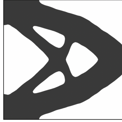
Figure 11: Three holes cantilever, steady case
