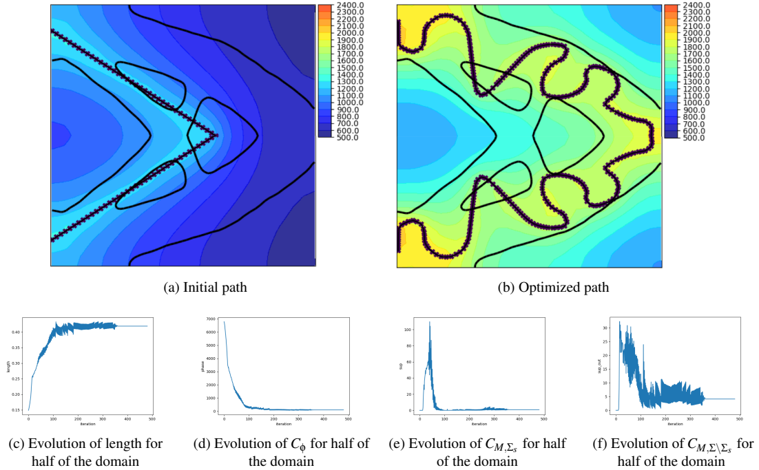
Figure 14: Initial and final temperature distribution as well as convergence histories, path optimization for the three holes cantilever from a hat initialization ( \eta = 5d_{lower} )
