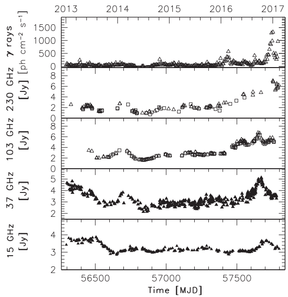
Figure 13. Multifrequency light curve for the period 2013 January 1–2017 February 9 in the following energy bands (from top to bottom): \gamma -rays (100 MeV–300 GeV; five-day time bins, in units of 10^{-8} ph cm ^{-2} s ^{-1} ; Fermi -LAT data), 230 GHz (in units of Jy; triangles: SMA data, squares: IRAM data), 91 and 103 GHz (in units of Jy; ALMA data), 37 GHz (in units of Jy; Metsähovi data), 15 GHz (in units of Jy; OVRO data).
