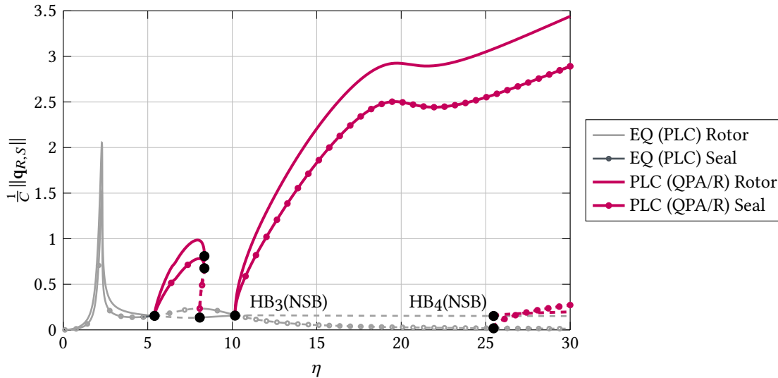
Figure 9. Bifurcation path for \kappa^2 = 7 and mass eccentricity e = 0.15 C ; normed rotor/ seal \frac{1}{C} \|\mathbf{q}_{R,S}\| radii are plotted against \eta = \frac{\Omega}{\omega_R} ; dashed lines indicate unstable solutions; all results wrt \mathcal{R} .
