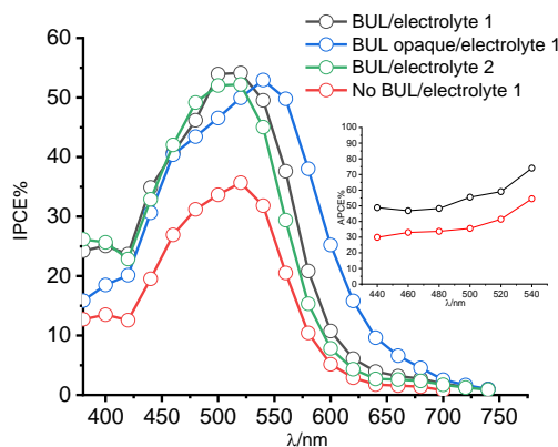
Figure 2. IPCE of TiO 2 based C1 sensitized solar cells collected under short circuit in the presence of I - /I 3 - based electrolytes. APCE spectra with BUL/e/1 (black) and No BUL/e/1 (red) are shown as inset
