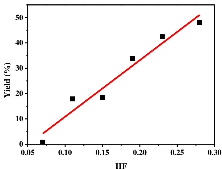
Fig. 12. The correlation between IIF and the isoheptane yield of catalysts.
