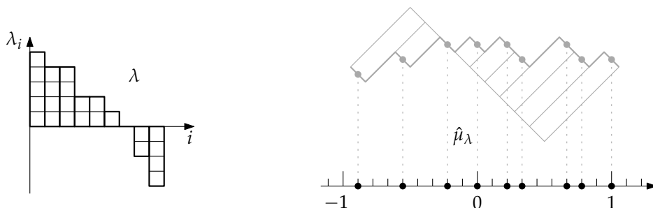
FIGURE 6. With N = 9 , the highest weight \lambda = (5, 4, 4, 2, 2, 1, 0, -2, -4) drawn in the style of a Young diagram, and its empirical measure. Each dot represents \frac{1}{9} of mass and any two dots are distant by a multiple of \frac{1}{9} .
