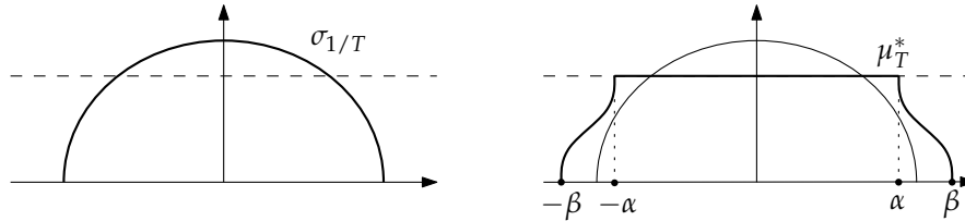
FIGURE 7. For T > \pi^2 , the absolute minimiser of the functional \mathcal{J}_T does not belong to the class of probabilities on \mathbb{R} with a density not exceeding 1. The minimiser within this class is represented on the right. Its density is identically equal to 1 on an interval in the middle of its support, and given by elliptic functions outside this interval.
