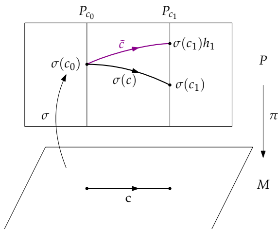
FIGURE 1. The difference between the horizontal lift of c starting at \sigma(c_0) , denoted in this picture by \tilde{c} , and \sigma(c) , the image of c by the local section \sigma , is measured by the function h which solves (5).
