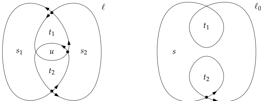
FIGURE 12. We are interested in computing \Phi(\ell) . The strategy is to use the Makeenko–Migdal equations to compute \partial_u \Phi(\ell) . As u = 0 , the two inner windings of \ell disentangle, and \ell becomes identical to \ell_0 . This loop \ell_0 is similar to the loop that we studied in Section 2.3, and becomes exactly this loop when t_2 = 0 . Our first task is thus to compute \partial_{t_2} \Phi(\ell_0) .
