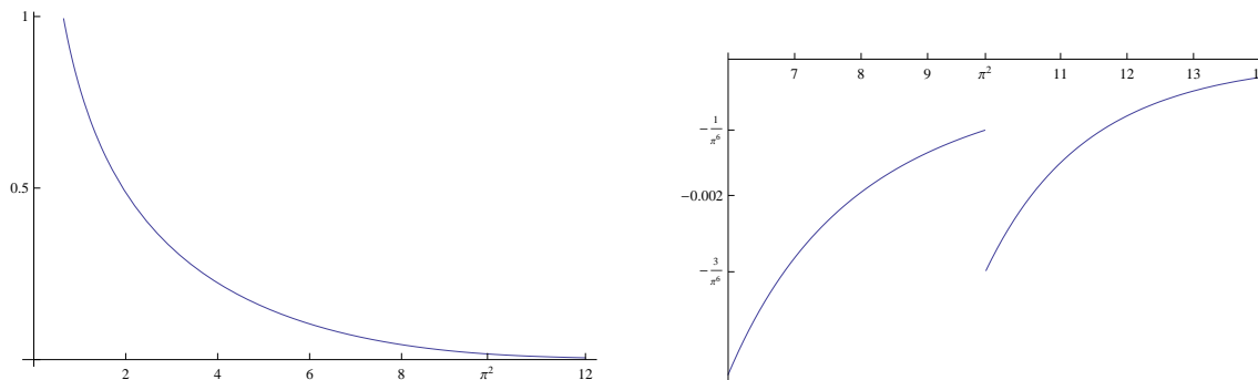
FIGURE 8. The graphs of T \mapsto F(T) (on the left) and of T \mapsto F^{(3)}(T) near T = \pi^2 (on the right).
