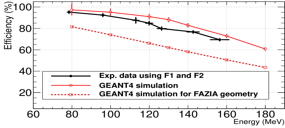
Figure 8: (Color on line) The experimental identification efficiencies (black symbols) according to the selection described in the text compared with a GEANT4 simulation (red open dots) both in the collimated geometry. Open squares correspond to a GEANT4 simulation for the uncollimated geometry of FAZIA detectors. Connecting lines are used to guide the eye.
