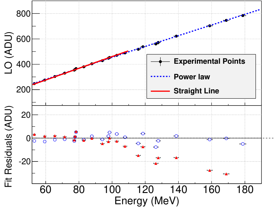
Figure 3: (Color on line) Upper panel: experimental correlation between the Light Output ( LO ) expressed in ADC unit (ADU) and the proton energy (black points) for the F1 crystal. The red line represents a linear fit of the experimental points below 110 MeV while the blue dotted line is a power law fit applied on the whole set of data (see text). Bottom panel: residuals of the two fits (red triangles: linear fit, blue open dots: power law). Note that for the linear fit the residuals are presented also for experimental points non included in the fit. Uncertainties are discussed in the text.
