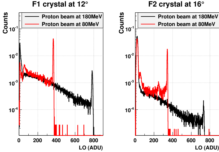
Figure 2: (Color online) Proton Light Output (LO) spectra expressed in ADC unit (ADU), measured with the two FAZIA CsI(Tl) in the collimated configuration at two beam energies. Left: detector F1 placed at 12^\circ with respect to the beam direction; Right: detector F2 placed at 16^\circ with respect to the beam direction. The histogram areas are normalized to 1.
