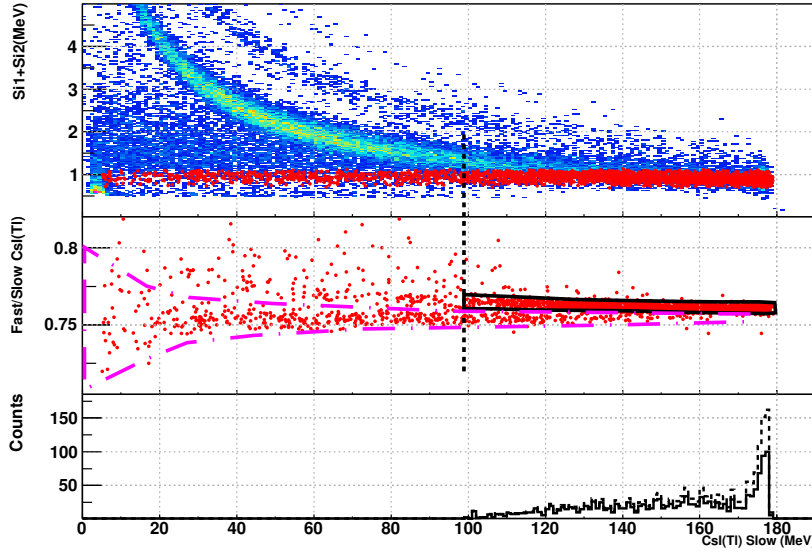
Figure 7: Top panel: \Delta E - E correlation for the F2 telescope already shown in Fig. 4, where the red points correspond to the selection of the N_{in,el} events explained in the text. Middle panel: the same events shown as red points in the upper part are presented in the \frac{FLO}{LO} vs E_{CsI} correlation. The colored contours are explained in the text. Bottom panel: energy distribution of the events with complete energy deposition selected by the black contour without (black line) and with (dotted line) efficiency correction (see text). Note that the beam energy is 180 MeV, but the low energy tail shifts the centroid of the distribution to \approx 157 MeV.
