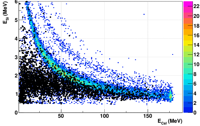
Figure 6: \Delta E-E correlation for protons at 180 MeV beam energy detected in the F2 telescope. The black points correspond to events falling within the dotted-magenta contour in Fig. 5.
