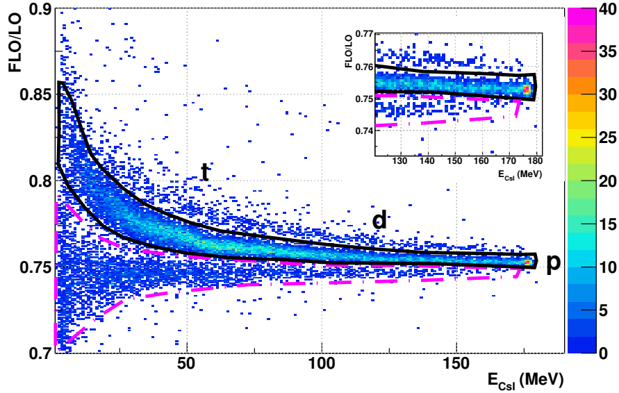
Figure 5: Matrix \frac{FLO}{LO} vs E_{CsI} for the crystal F2 measured at 180 MeV beam energy. The dotted-magenta contour is explained in the text. The black contour includes the properly identified protons. An expanded view of the region close to the elastic peak is also shown.
