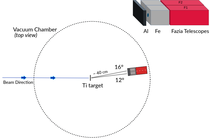
Figure 1: Layout of the experimental set-up. The iron collimators (Fe) and the aluminium (Al) absorber are shown. They are placed in front of the two FAZIA telescopes during part of the operation – see text for details.
