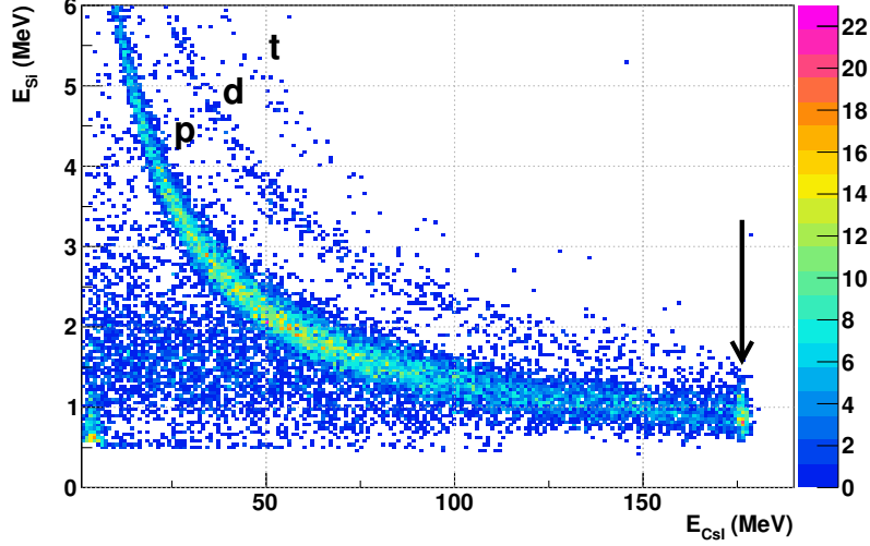
Figure 4: The sum of the energies deposited in the two silicons vs. LO correlation for the crystal F2 in the case of 180 MeV proton beam. The vertical arrow indicates the proton elastic peak, while letters indicate the ridges of the Hydrogen isotopes. Only events with an energy deposition in Silicon detectors higher than the noise level are reported. Residual events due to \gamma -rays are present on the bottom left-hand side (see text).
