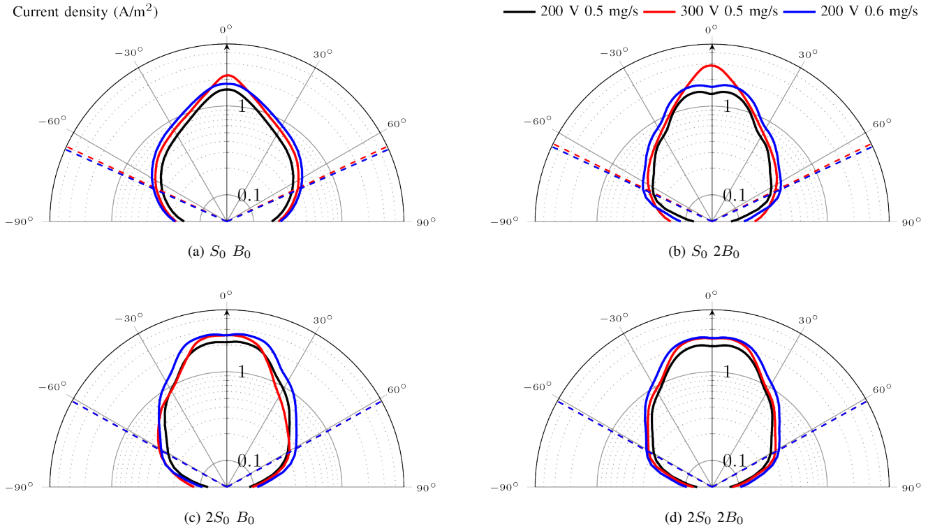
Fig. 4. Current density profiles across the plume of each configurations at 200 V 0.5 mg/s, 300 V 0.5mg/s and 200 V 0.6 mg/s operating conditions. The dashed lines represent the computed divergence angle \alpha_d .
