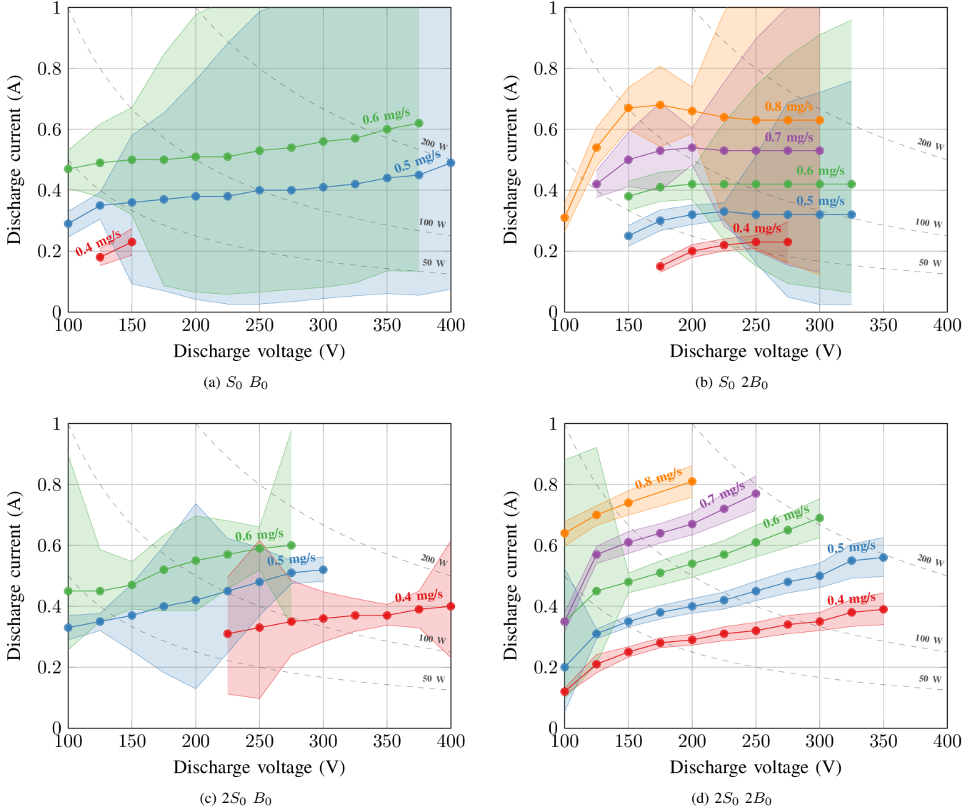
Fig. 3. ISCT100 Hall thruster discharge current as a function of anode mass flow rate and discharge voltage for different configurations.
