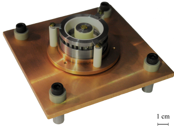
Fig. 1. Photograph of the 100 W-class permanent magnet ISCT100 Hall thruster developed at ICARE. The external cathode is not shown.
