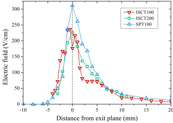
Fig. 5. Electric field measured by LIF at 200 V in the 100 W ISCT100 ( 2S_0 2B_0 ) and the 200 W ISCT200, and at 250 V in the 1.3 kW SPT100.
