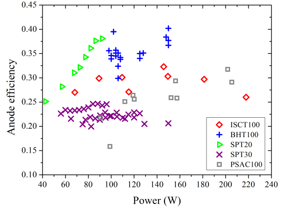
Fig. 7. Comparison of the anode efficiency of 100 W class low power Hall thrusters (BHT-100 [34], SPT-20 [35], SPT-30 [19], PSAC 100 [36])
