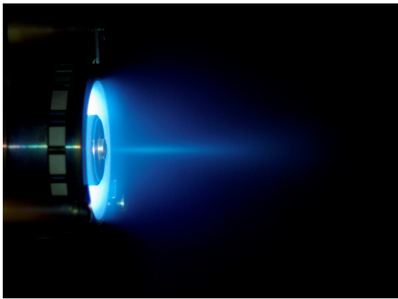
Fig. 2. ISCT100 Hall thruster in 2S_0 B_0 configuration firing with xenon at 100 W input power. The residual gas pressure in the vacuum chamber is 4 \times 10^{-5} mbar.
