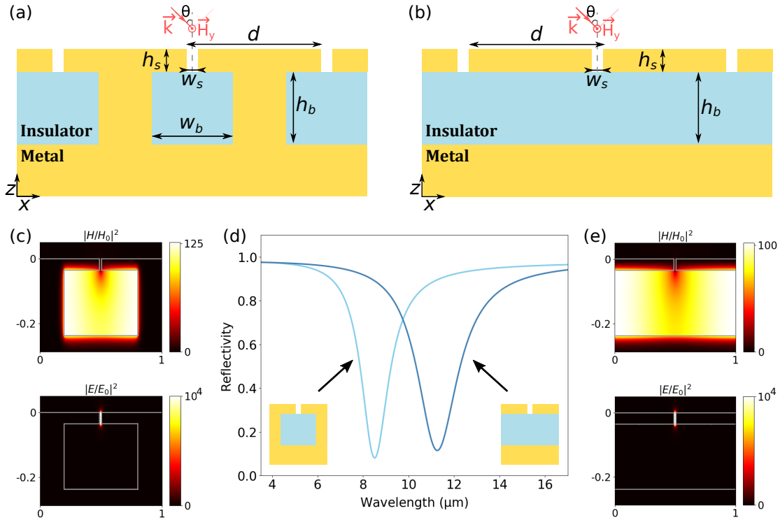
Fig. 1: (a) The optical Helmholtz resonator consists in a metallic slit-box structure. (b) The optical Helmholtz-like resonator is obtained in the asymptotic case where the boxes have their width w_b equals to the period d . (d) Comparison of infrared spectra in TM polarization of two resonators whose box widths are: w_b = 600 nm and w_b = 1 \mu m. The other dimensions are identical: d = 1 \mu m, h_b = 200 nm, h_s = 37 nm and w_s = 12 nm. For both resonators, the box is filled with a dielectric material of permittivity \epsilon = 4.84 . (c) and (e) Maps of the magnetic and electric fields at the resonance, respectively for both resonators whose spectra are shown on (d).
