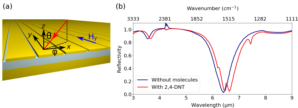
Fig. 2: (a) Three dimensional representation of an Helmholtz-like resonator with an incoming plane wave with the polar angle \theta and the azimuthal angle \phi . (b) Infrared reflection spectra of resonators, whose dimensions are d = 3 \mu\text{m} , w = 300 \text{ nm} , h_s = 100 \text{ nm} and h_b = 50 \text{ nm} , without (blue line) and with 2,4-DNT (red line).
