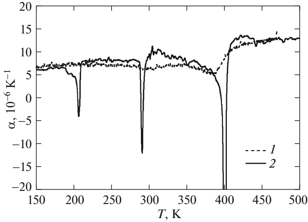
Fig. 4. Temperature dependences of the thermal expansion coefficient for (1) the nBT and (2) mBT ceramic samples.
