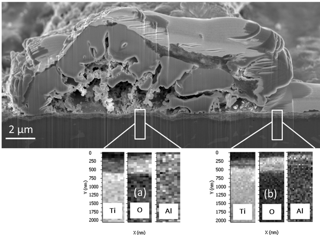
Figure 3 FIB SEM cross section and Auger mapping of the DMAI500 sample after oxidation during 5000 h at 600 °C. a Area under an “excrescence”, b area without “excrescence”.
